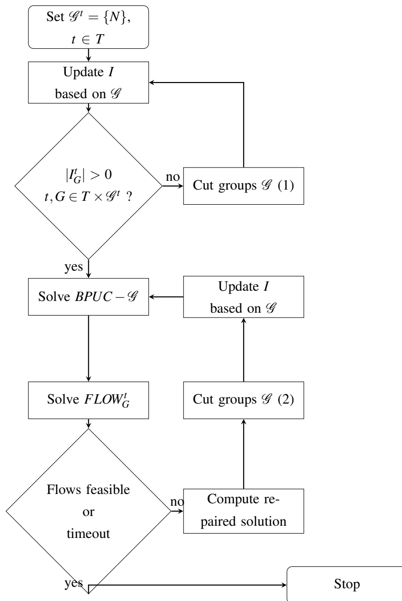
Figure 6.5: IAD flowchart
