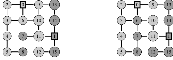
Figure 3.1: Solutions of (3.1)-(3.6)
