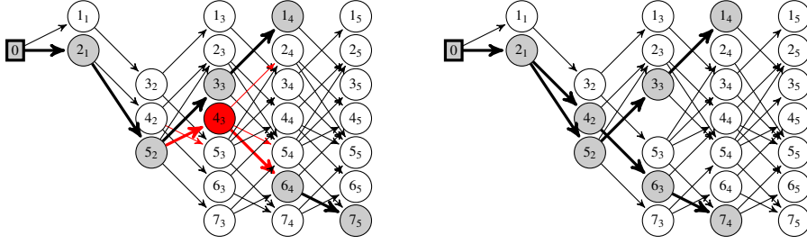
Figure 3.5: Triangle reductions
