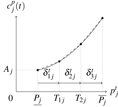
Figure 2.2: Production cost of a thermal generator
