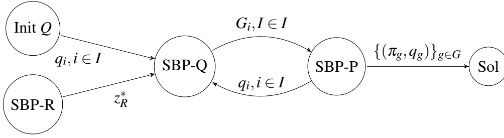
Figure 5.9: SHBP
