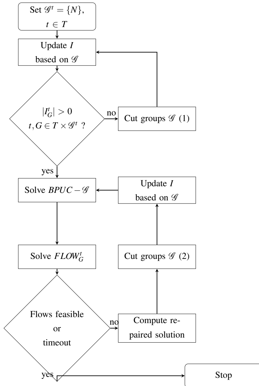
Figure 6.5: IAD flowchart
