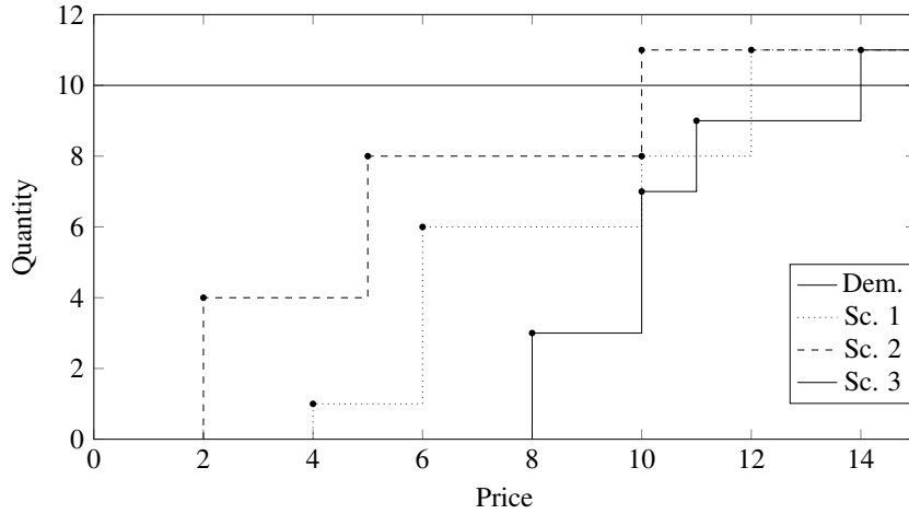
Figure 5.1: BP instance
