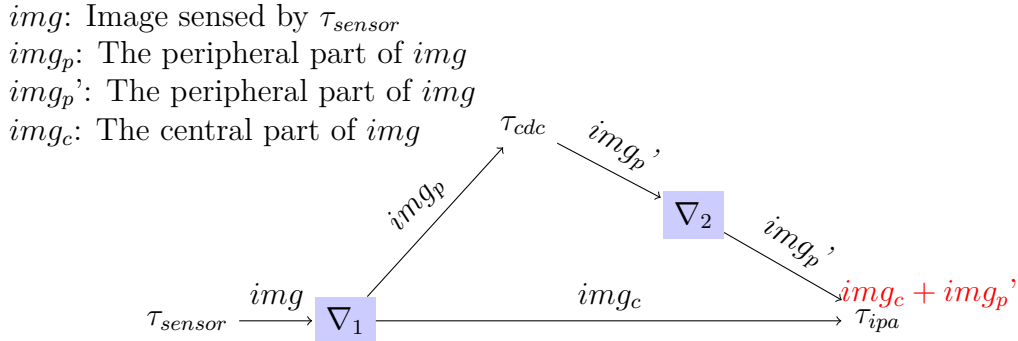
Figure 1.16: Data matching motivating example.
