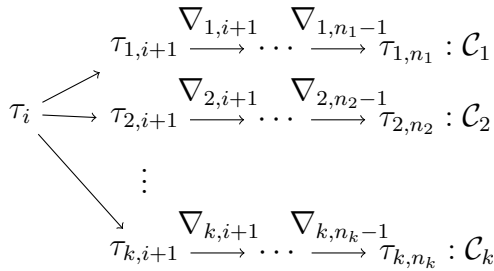
Figure 1.13: Example of k diverging functional chains.
