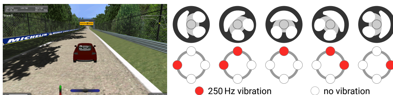
Figure III.4 – Screenshot of the customized version of VDrift, an open-source car racing game. The right side shows the mapping of the vibrotactile feedback depending on the steering angle.
