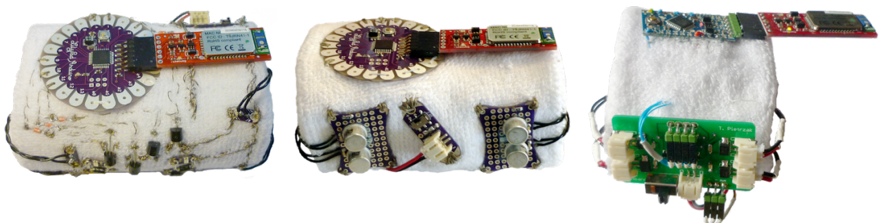
Figure III.2 – Three iterations of haptic wristband prototypes. On the first prototypes, components were connected with conductive thread. On the second prototype, the components were soldered on protoboards that were connected with conductive thread. The third prototype used a homemade PCB connected with wires.
