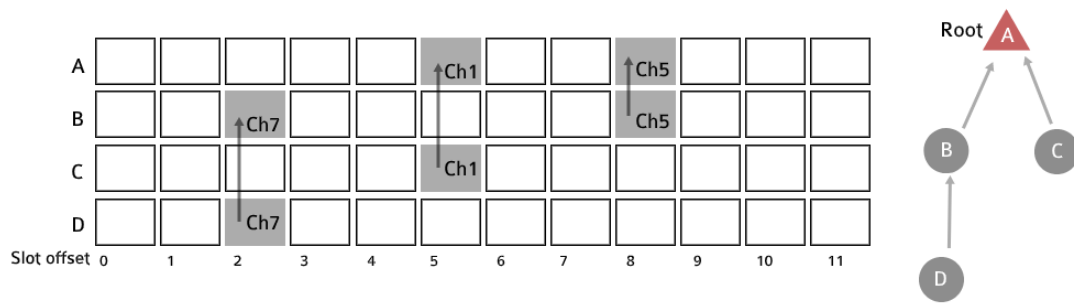
Figure 1.3: A typical TSCH slotframe for Motes A–D, using a uniform slot duration and single PHY at a fixed bitrate. Each node allocates a specific slot offset and channel offset for transmissions to its parent.
