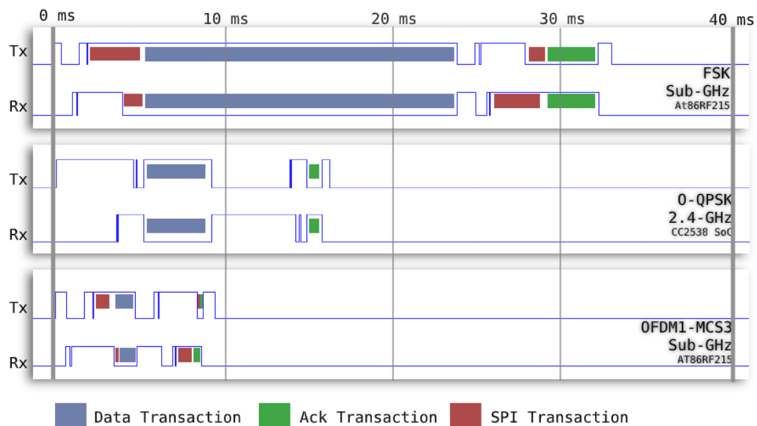
Figure 4.1: Timeslot templates for the three PHYs, for a 100 B data payload with acknowledgment. Red markers highlight when SPI transactions between the micro-controller and the AT86RF215 take place.
