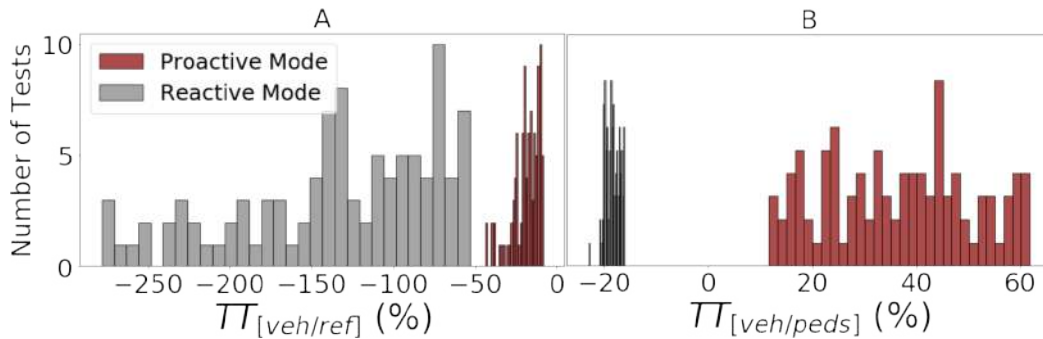
Fig. 4.7.: Histogram of the vehicle's relative travel time. A: TT_{[veh/ref]} , B: TT_{[veh/peds]}
