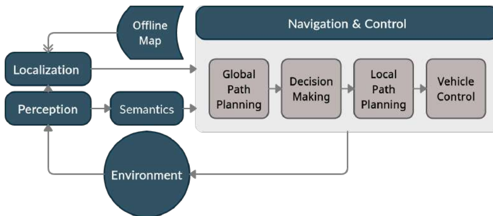
Fig. 2.5.: The autonomous vehicle system components
