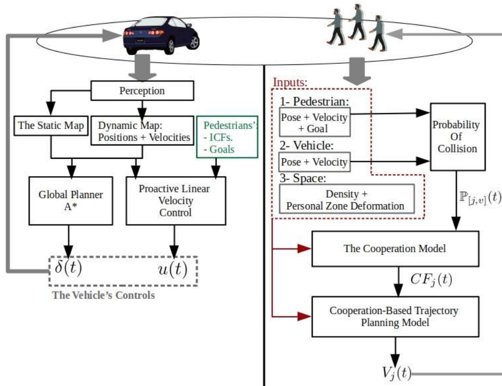
Fig. 8.2.: The longitudinal proactive controller implementation summary
