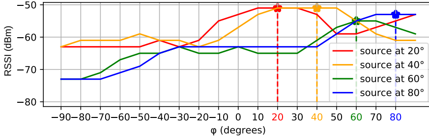
Figure 4.10: Sweeping along the \varphi axis to locate the source. The source position is found when maximum RSSI is measured
