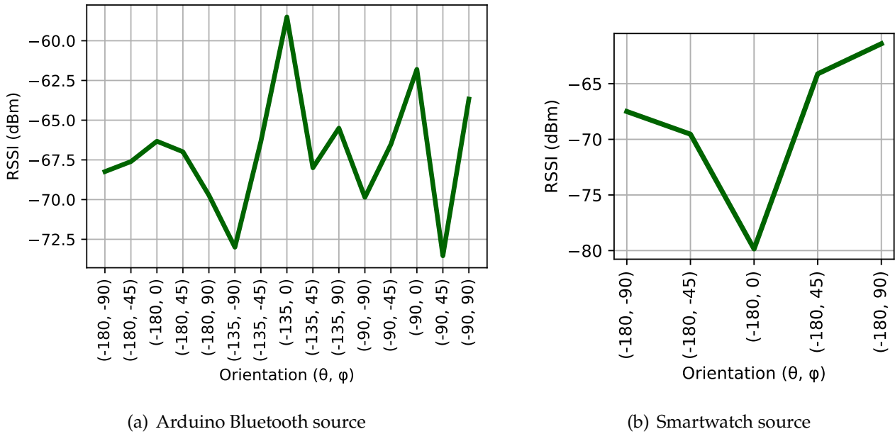
Figure 4.19: Sensitivity of the Bluetooth RSSI to the device orientation in an office environment. We observe a large variability of the RSSI with the device orientation for both sources.
