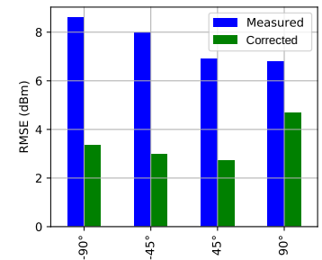
Figure 4.13: RMSE for different source orientation of the main lobe between the reference RSSI and the raw RSSI measurements (in blue), and the reference RSSI and the corrected RSSI measurements (in green). The impact of the source orientation on the measured LTE RSSI can be accounted for and corrected.
