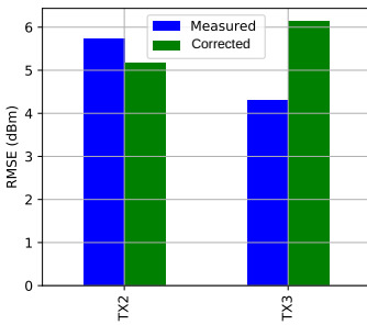
Figure 4.15: Root Mean Squared Error (RMSE) for different source Tx power between the reference RSSI and the raw RSSI measurements (in blue), and the reference RSSI and the corrected RSSI measurements (in green). The impact of the source Tx on the measured LTE RSSI cannot be corrected with the mere application of the calibration matrices.
