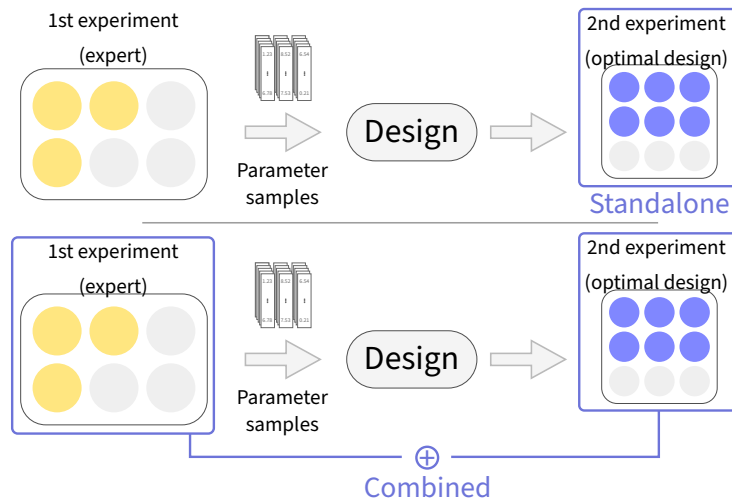
Figure 6.2.: Our two kinds of designs, either Top: standalone or Bottom: combined. The blue box indicates what experiments are used for the final fit.
