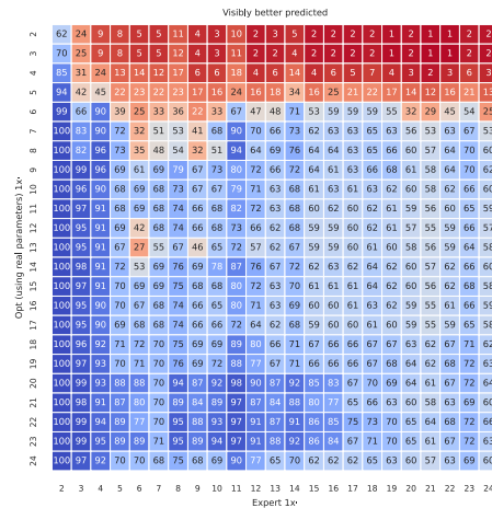
Figure 5.10.: Same as Figure 5.9-Left, but no error is considered negligible. Still, the optimal design beats the expert once afforded enough wells.
