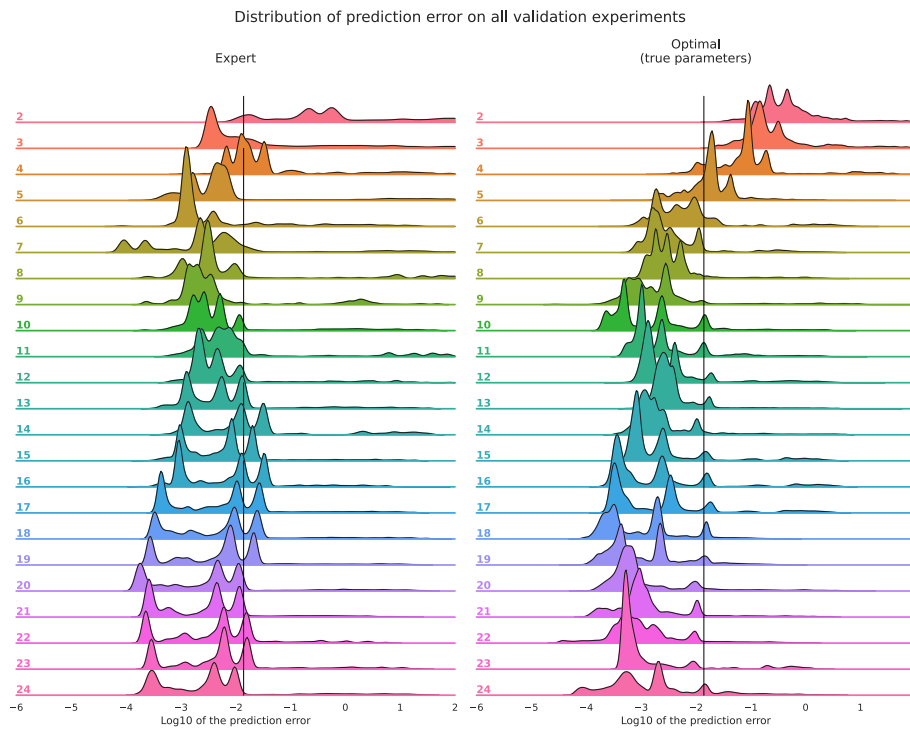
Figure 5.8.: Distributions of the \log_{10} of the prediction error across all validation experiments, for the expert designs and the optimal designs computed with the true parameters. The number of parallel experiments is indicated on the left (from 2 to 24). The solid black vertical line indicate the threshold below which the error is considered negligible.
