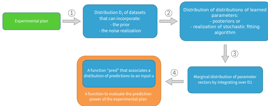
Figure 4.4.: A flow chart representing the general process of assessing the quality of an experimental plan. 1: The experimental plan is used to simulate datasets. The datasets can vary because we currently have a distribution of estimates of the true parameters of the system, or because of different realizations of the noise stochastic process. 2: For each of these datasets, we can use a (to-be-defined) learning method to obtain a corresponding distribution of parameters. Because we had a distribution of datasets, we obtain a distribution of distributions of parameters. 3: We marginalize the previous distribution to obtain a distribution of parameters. 4: We now have a distribution of parameters that could be learned from the experimental plan, and we want to assess its prediction power. To each input u , we can associate a distribution of prediction of the system's dynamic corresponding to each parameter of our distribution from step 3. We can then use this function to compute some numerical score of prediction power.
