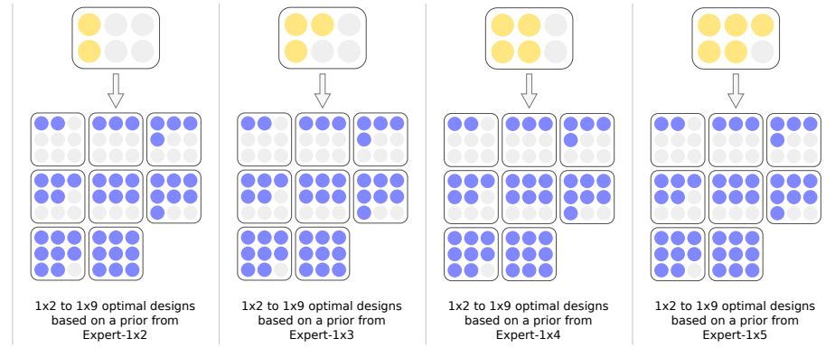
Figure 6.1.: Graphical summary of the iterative design setup: four expert designs can be used as a first learning step, and parameters obtained by learning on them are then used to design eight optimal designs.
