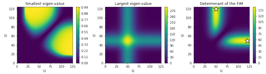
Figure 3.4.: Left and center: Smallest and largest eigenvalue of the FIM, for varying sampling times t_1 and t_2 . Right: Product of the eigenvalues (also the determinant of the FIM). White stars indicate the (symmetrical) maximum, the corresponding sampling times (50min and 120min) maximize the information (according to the D-criterion)
