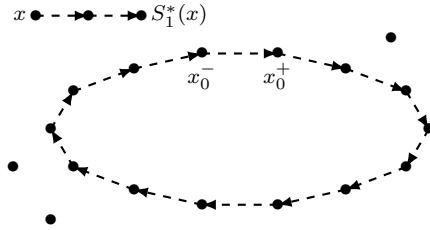
Figure 3.6: After the greedy part of Algorithm 5, with one frequent type.
