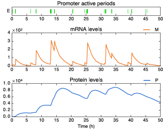
Figure 1.9. Illustrative simulation of the two-state model for a single gene. Top panel describes the activity of the promoter (green spike means the promoter is "ON", no bar means it's "OFF"). Middle panel presents the associated mRNA levels over time (h), while the bottom panel visualizes the corresponding effect on the protein level. From Herbach et al. [159].
