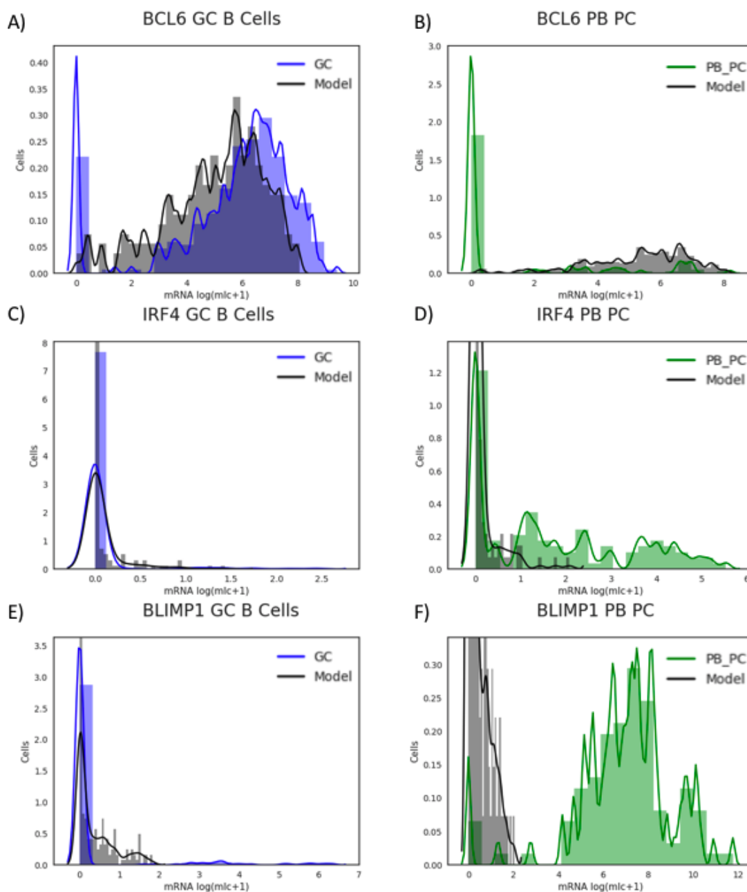
Supplementary Figure S4. The Kernel Density Estimate (KDE) plot and histograms of model-generated and experimental mRNA counts of BCL6, IRF4, BLIMP1 at GC and PB_PC stages. The subgraphs A, C, E represent log (molecule+1) normalized SC with BCL6, IRF4 and BLIMP1 compared between the model estimations at GC stage (grey) vs the experimental data from GC B cells (blue). The subgraphs B, D, F represent log (molecule+1) normalized SC with BCL6, IRF4 and BLIMP1 compared between the model estimations at PB_PC stage (grey) vs the experimental data from PB_PC cells (green). Simulation of 200 SC were used based on the parameter set, selected after automatized parameter screening strategy (see Tables 2.2-2.5, version II). Performed based on dataset from Milpied et al. [3]
