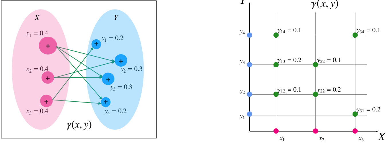
Figure 3.1: Kantorovich's transport plan between two discrete distributions of masses defined on spaces X and Y , allowing to distribute mass from the one location to multiple locations.
