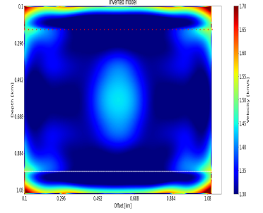
S_{\varepsilon,\lambda} -inv
