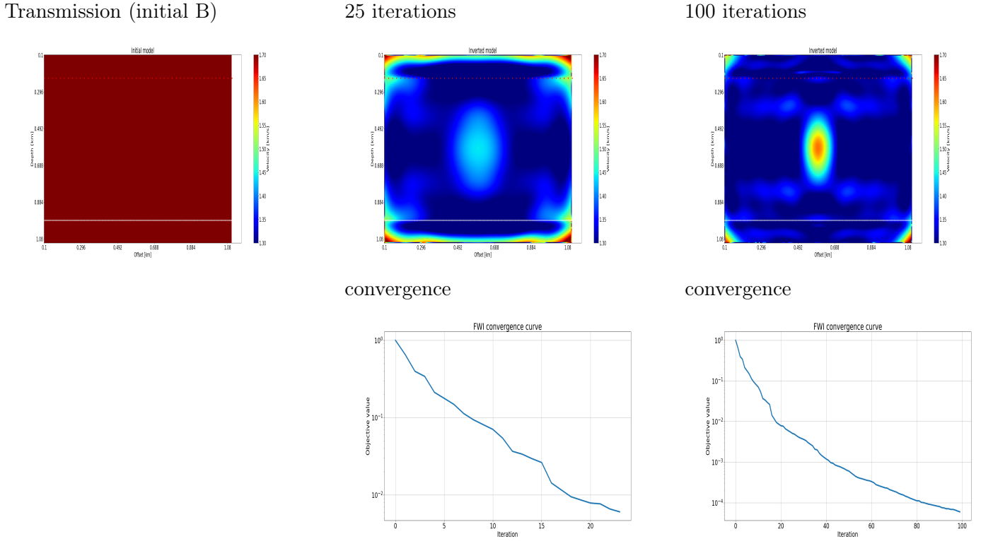
Figure 6.3: S_{\epsilon, \lambda} inversion: transmission (initial model B)
