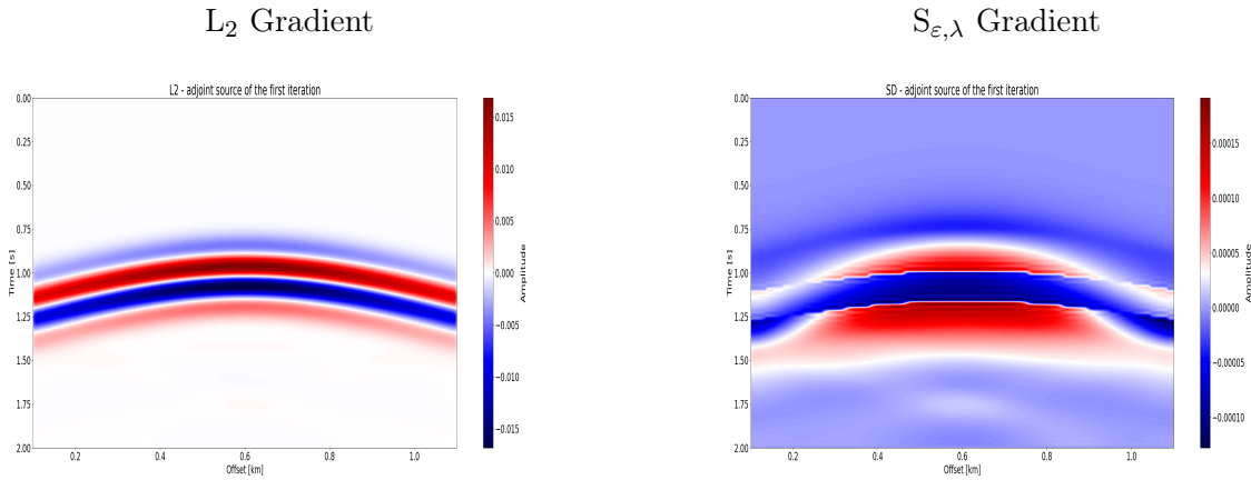
Figure 6.10: Ajoint-source in the time-receiver domain at the first FWI iteration.
