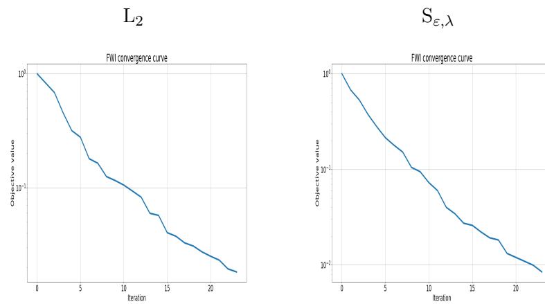
Figure 6.26: Convergence rate of the L_2 (left) and S_{\varepsilon,\lambda} (right) based inversion
