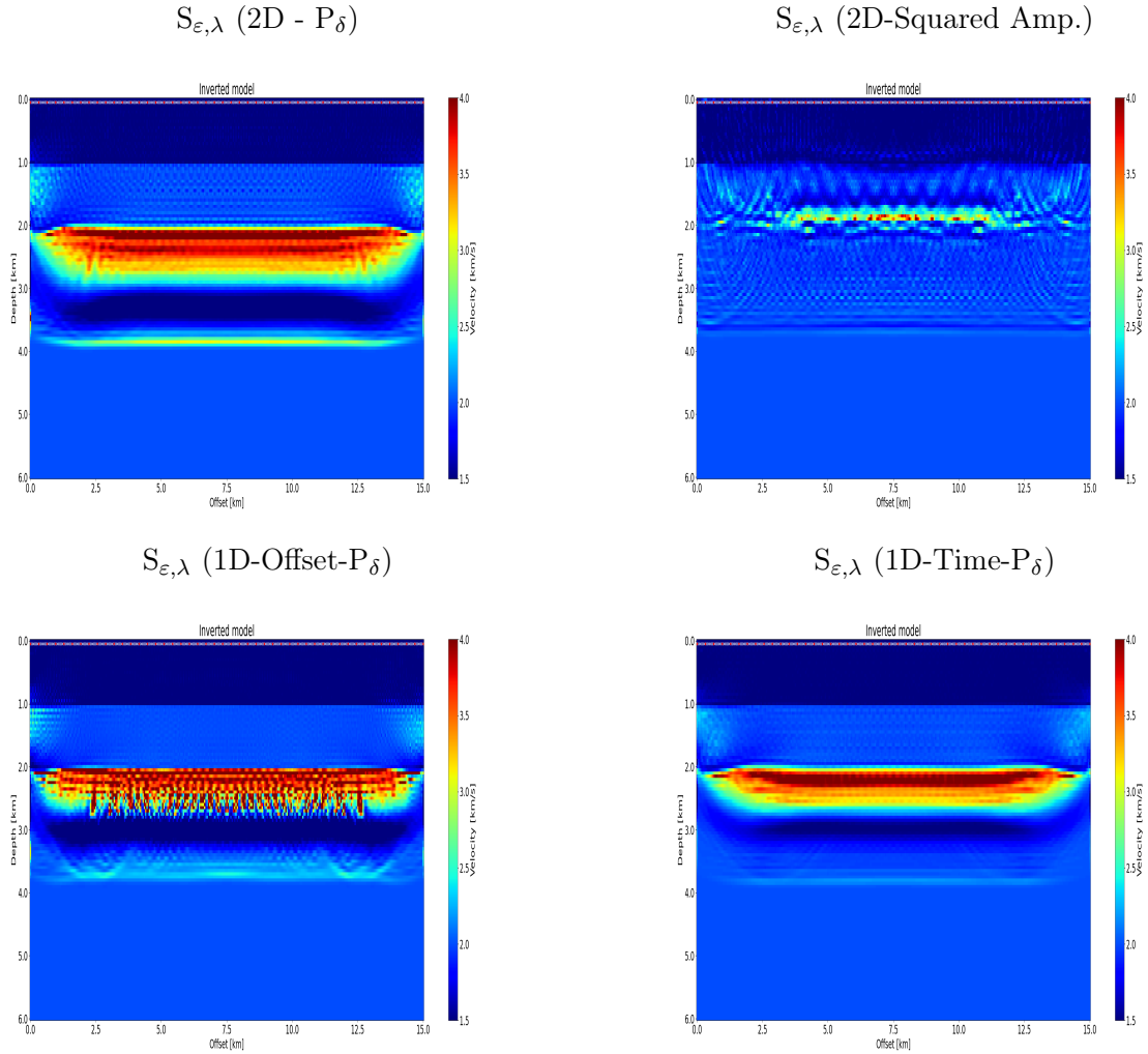
Figure 6.47: Reconstructed models for different implementation strategies of the S_{\epsilon,\lambda} -misfit function: 2-D transport after decomposition of the signals into positive and negative parts (upper-left figure); Squared-transform of the signals before 2-D transport (upper-right figure); 1-D transport in space (offset-by-offset) after decomposition of the signals into positive and negative parts (lower-left figure); 1-D transport in time (trace-by-trace) (lower-right figure). The later two implementations make use of the separability of the Gibbs matrix in the Sinkhorn algorithm and of the appropriate scaling of the transport domain.
