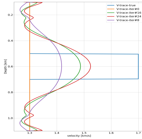
Figure 6.6: Velocity profile along a vertical section of the physical domain at a surface position x = 600 m as reconstructed by the S_{\epsilon,\lambda} based inversion.
