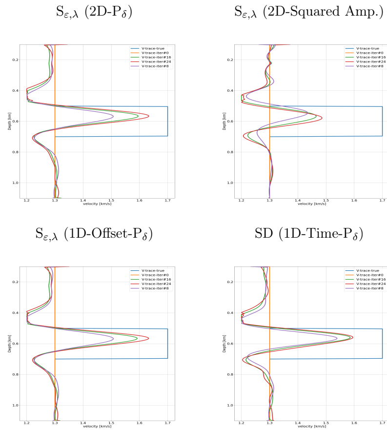
Figure 6.25: Velocity profile along a vertical section of the physical domain for different FWI iterations and different implementations of the S_{\varepsilon,\lambda} -misfit function.
