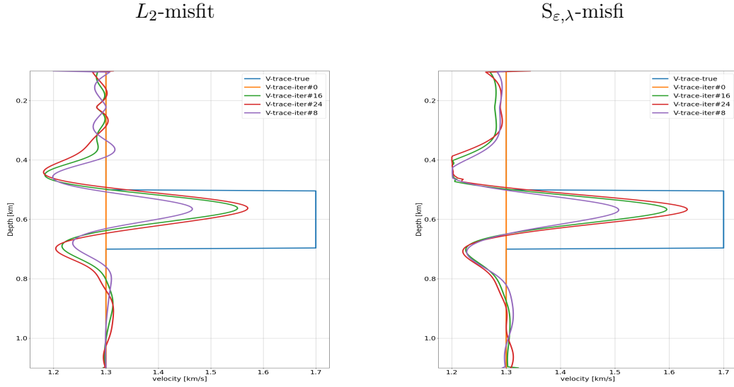
Figure 6.21: Velocity profile along a vertical section of the physical domain at surface position x = 600 m at different inversion iterations with the L_2 and the S_{\epsilon,\lambda} misfit functions.
