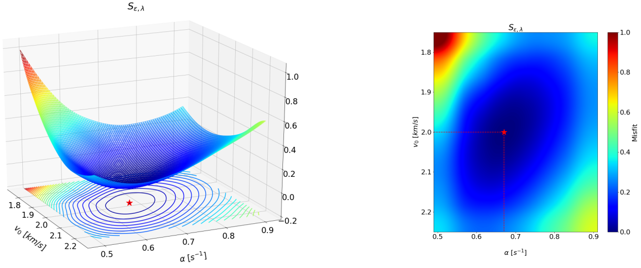
Figure 5.12: Misfit function based on the Sinkhorn divergence ( S_{\varepsilon, \lambda} ), with respect to v_0 and \alpha . The red star is the location of the global minimum, while the position of the reference model v_0^*, \alpha^* is indicated as the intersection of the two dashed lines.
