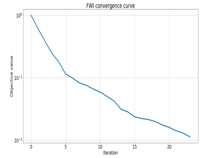
S_{\varepsilon,\lambda} -inv
