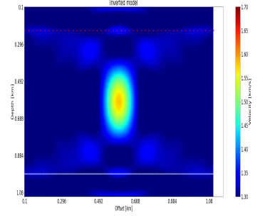
S_{\varepsilon,\lambda} -inv
