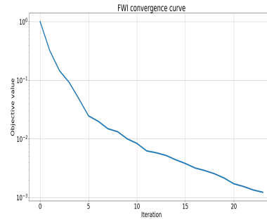
L_2 -inv
