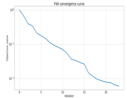
S_{\varepsilon,\lambda} -inv
