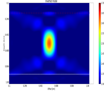
L_2 -inv
