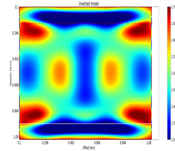
Figure 6.1: Numerical inversion after 25 iterations
