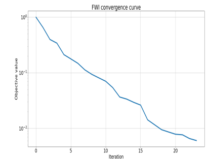
S_{\varepsilon, \lambda} -inv
