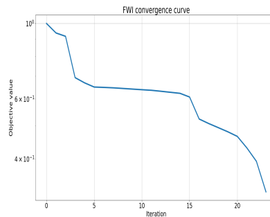
Figure 6.2: Inversion convergence
