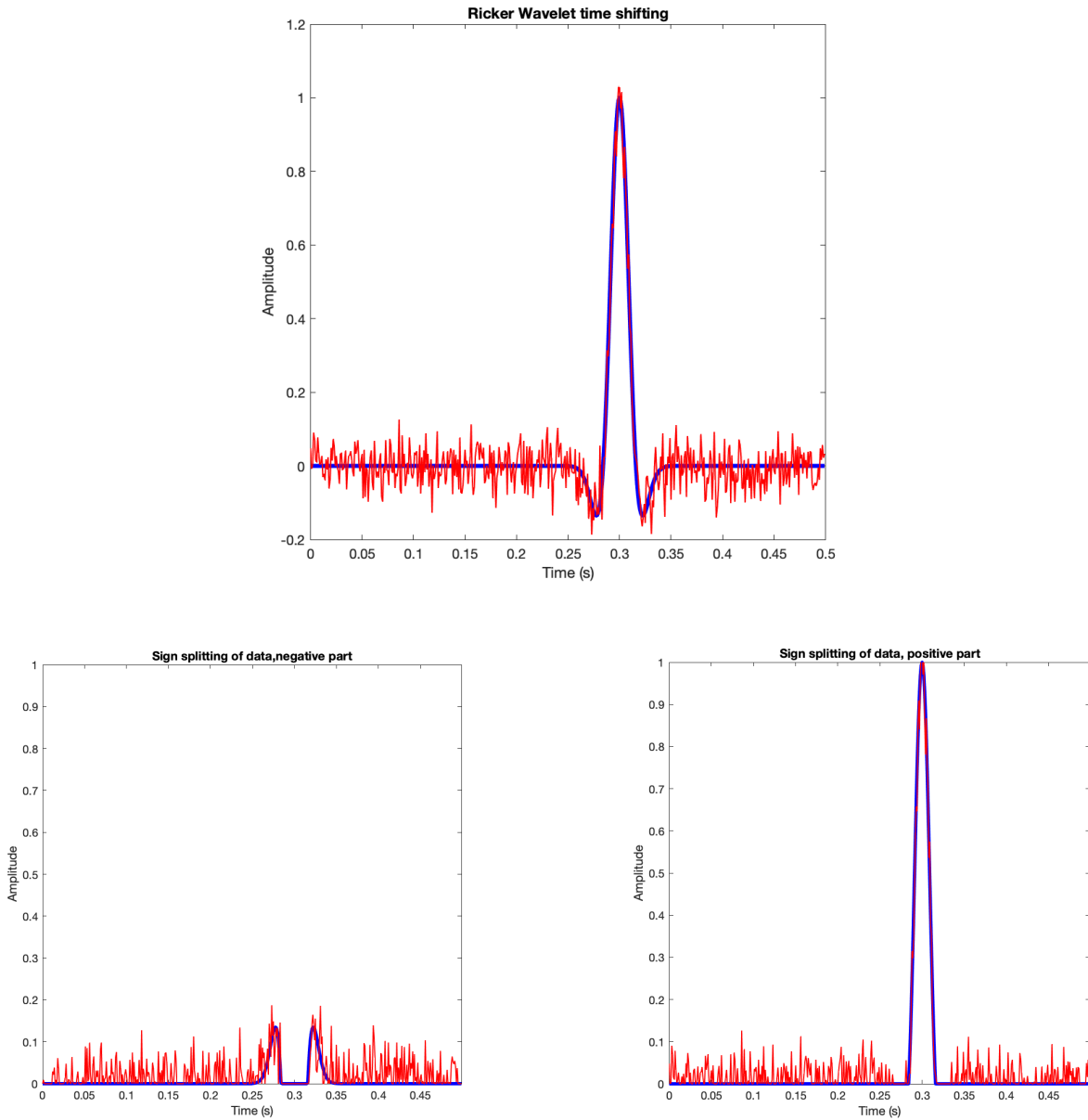
Figure 5.5: Top figure: Ricker wavelets g(t) (solid blue line) and f(t) (solid red line), with an added Gaussian noise. Bottom figures: the negative (bottom-left figure) and the positive (bottom-right figure) parts of the two Ricker wavelets.
