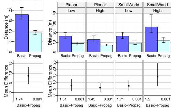
Figure 7. (Top) Average distance traveled by participant per TECH in the individual user case, aggregated on the left, and for each GRAPH × COMPLEXITY conditions on the right. (Bottom) Difference CIs for the analysis.
