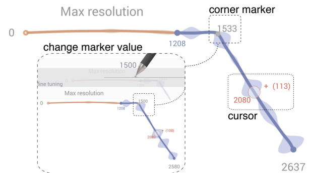
Figure 6. Corners can serve as markers of values of interest. As with extrema, the user can adjust the value of a corner by long-pressing and dragging its label along the horizontal axis. A slider cursor reveals both the value of its center and the number of active data points it covers.
