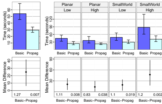
Figure 4. (Top) Average time to complete the task per TECH in the individual user case, aggregated on the left, and by GRAPH × COMPLEXITY conditions on the right. (Bottom) Corresponding 95% CIs for the mean differences Basic – Propagation used in analysis; bottom left numbers show the Cohen’s d effect size and the right ones the p values. This convention is followed in all images.
