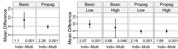
Figure 9. 95% CIs for mean differences of the traveled distance Individual – Multi-user , by TECH and TECH × COMPLEXITY.
