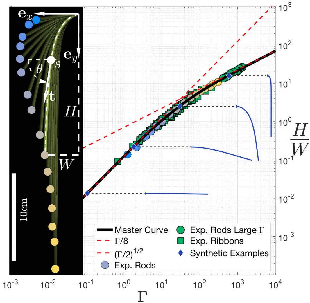
Fig. 3.5: Master curve and experimental validation for the Cantilever test . Left: snapshots of experimental rods under gravity, with 16 different \Gamma values. Right: our computed master curve (in black) representing the aspect ratio of the rod's shape as a function of \Gamma , together with experimental results from [Rom+21]
