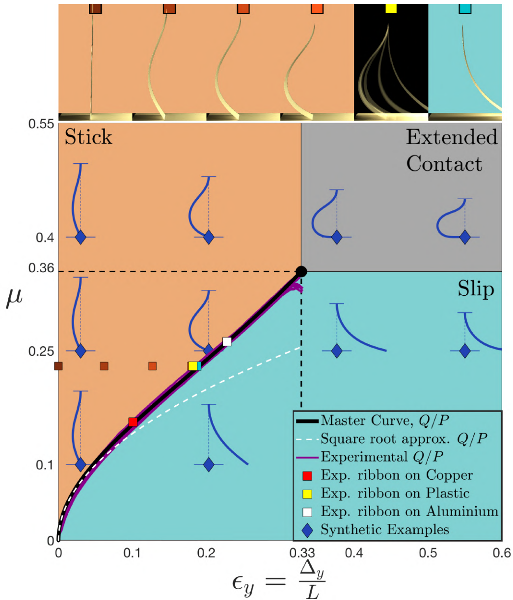
Fig. 3.2: Master curve and experimental validation for the Stick-Slip test. Phase diagram where the master curve (in black) separates the sticking regime (in orange) from the slipping regime (in teal). The extended contact region (in gray) is not used in our validation protocol. The (numerical) black and (experimental) purple curves are plots of the ratio Q/P as a function of \epsilon_y .
