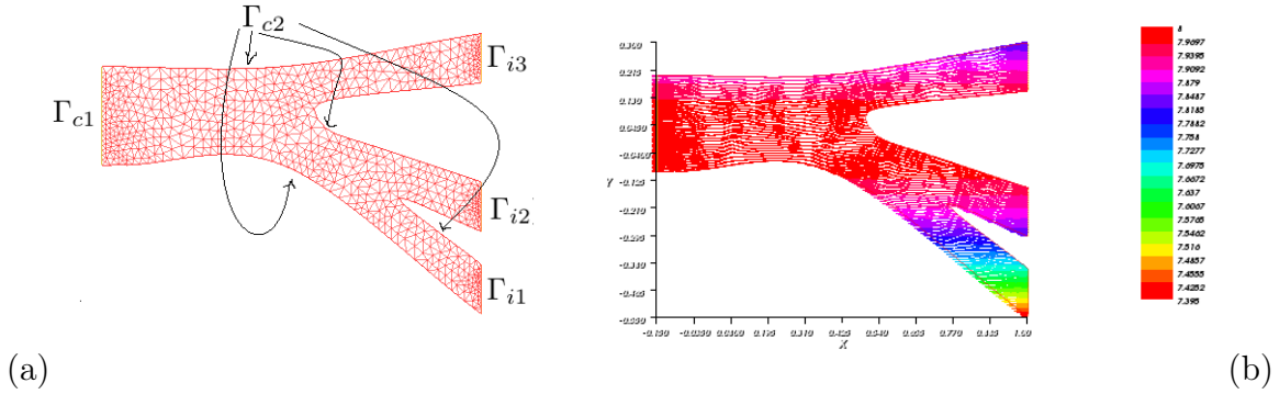
FIGURE 5.2 – Test case C. (Left) Mesh used for solving the coupled inverse problem. (Right) Iso-values of the velocity field.
