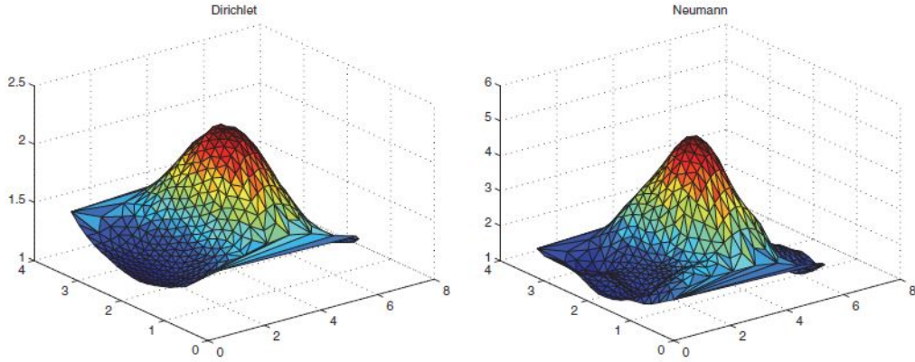
FIGURE 1.5 – Reconstructed nonradial Dirichlet ( \tau_N , left) and Neumann ( \eta_N , right) data over \Gamma_i . The profiles are presented at convergence and for a noise level \sigma = 5\% [56].
