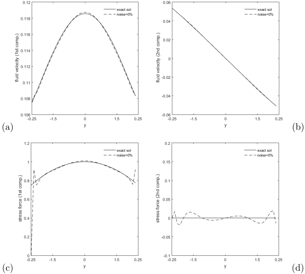
FIGURE 4.6 – Case B- Reconstruction of the missing boundary data (for unnoisy data). (a) exact -line- and computed -dashed line- first component of the velocity over F_i (b) exact -line- and computed -dashed line- second component of the velocity over F_i (c) exact -line- and computed -dashed line- first component of the normal stress over F_i (d) exact -line- and computed -dashed line- second component of the normal stress over F_i .
