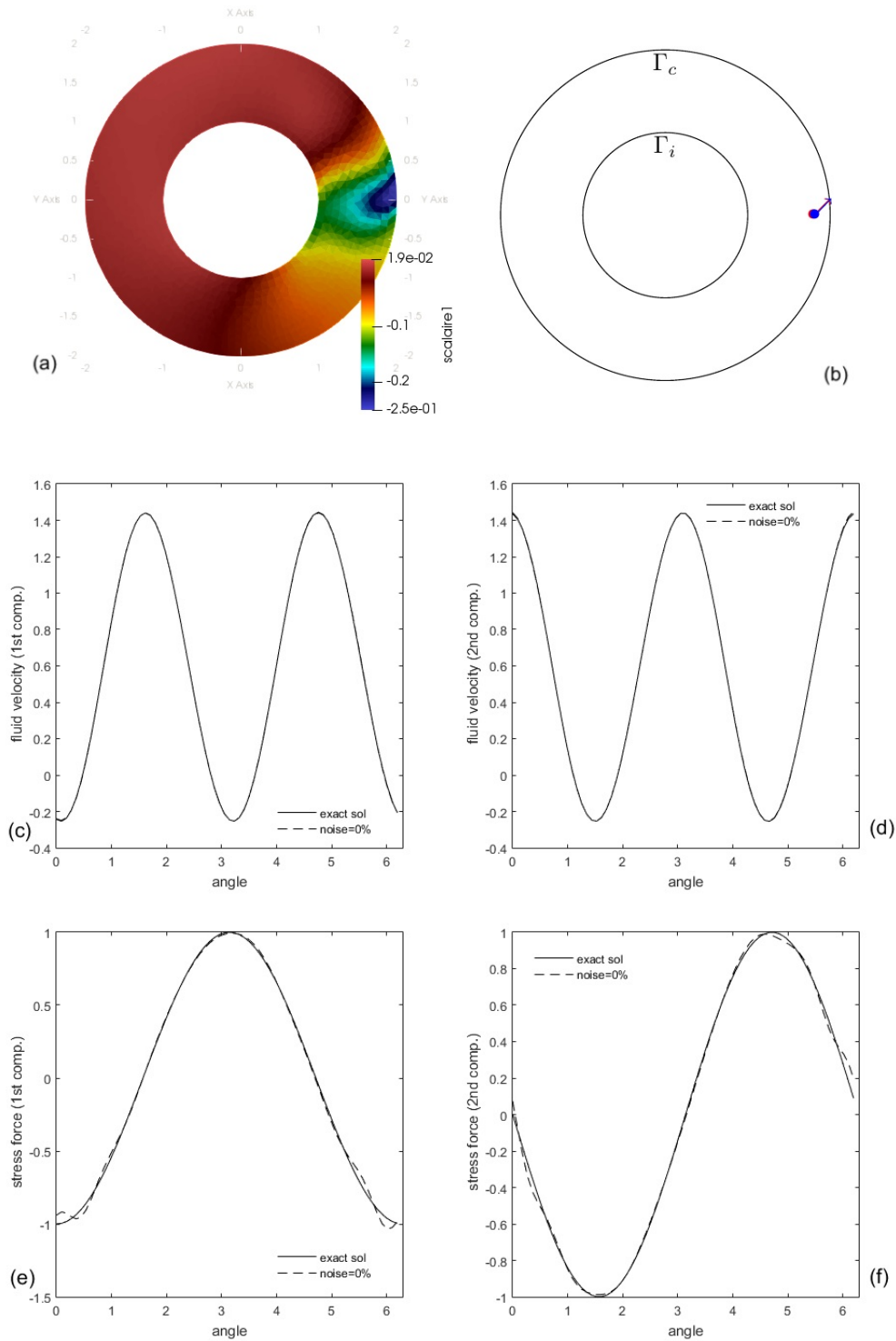
FIGURE 3.4 – Test case A. Reconstruction of the point-forces and missing boundary data with noise free Dirichlet data over \Gamma_c . (a) the iso-values of the topological gradient at convergence. (b) exact elements defining the source-term -red vector- and computed one -blue vector- (c) exact -line- and computed -dashed line- first component of the velocity over \Gamma_i . (d) exact -line- and computed -dashed line- second component of the velocity over \Gamma_i . (e) exact -line- and computed -dashed line- first component of the normal stress over \Gamma_i (f) exact -line- and computed -dashed line- second component of the normal stress over \Gamma_i .
