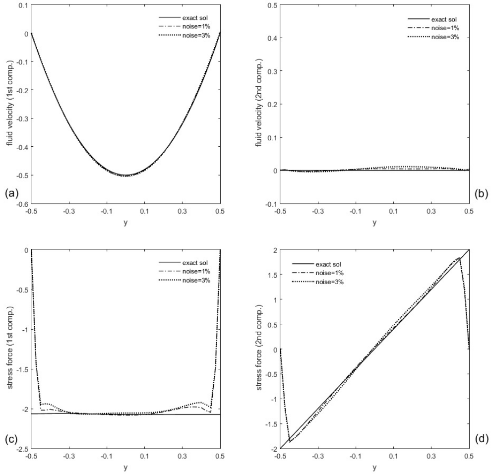
FIGURE 3.10 – Test case C. Reconstruction of the missing boundary data with noisy Dirichlet data over I_c with noise levels \sigma = \{1\%, 3\%\} . (a) exact and computed first components of the velocity over I_i (b) exact and computed second components of the velocity over I_i (c) exact and computed first components of the normal stress over I_i (d) exact and computed second components of the normal stress over I_i .
