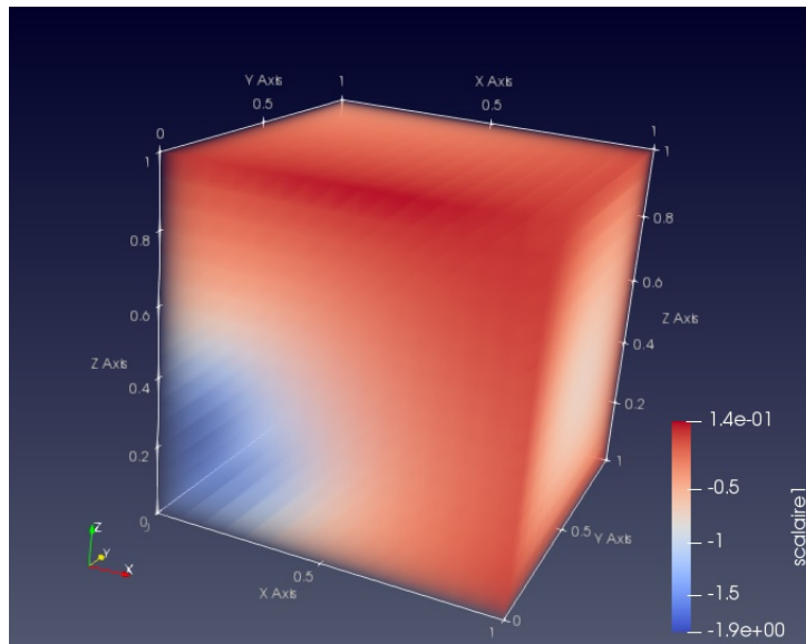
FIGURE 3.11 – The iso-values of the topological gradient at convergence, P_{op} = (0.2, 0.2, 0.2) and \Lambda_{op} = (0.233, 0.204, 0.005) . Exact values : P_{ex} = (0.25, 0.25, 0.25) and \Lambda_{ex} = (0.25, 0.2, 0) .
