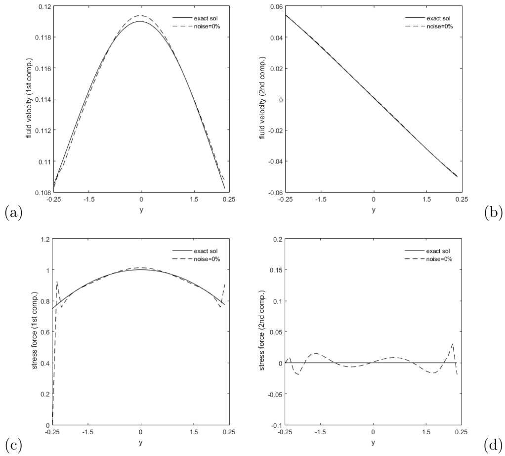
FIGURE 4.4 – Case A- Reconstruction of the missing boundary data (for unnoisy data). (a) exact -line- and computed -dashed line- first component of the velocity over I_i^r (b) exact -line- and computed -dashed line- second component of the velocity over I_i^r (c) exact -line- and computed -dashed line- first component of the normal stress over I_i^r (d) exact -line- and computed -dashed line- second component of the normal stress over I_i^r .
