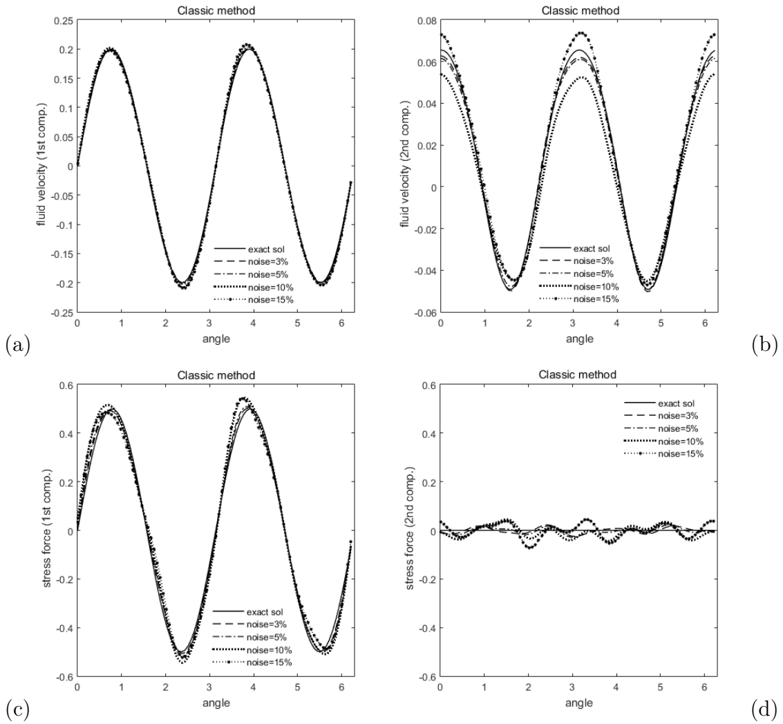
FIGURE 5.5 – Test case-A "Classic Method". Reconstruction of the missing boundary data with noisy Dirichlet data over L_c with noise levels \sigma = \{3\%, 5\%, 10\%, 15\%\} . (a) exact and computed first components of the velocity over L_i (b) exact and computed second components of the velocity over L_i (c) exact and computed first components of the normal stress over L_i (d) exact and computed second components of the normal stress over L_i (w.r.t a uniform noise).
