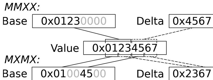
Figure 6.8 – Mapping deltas to different positions of the values. M is a base byte, and X is a delta byte. When using mapping MMXX (top), the deltas are calculated relative to the last two bytes of the values. When using mapping MXMX (bottom), deltas are relative to the first and third least-significant bytes.
