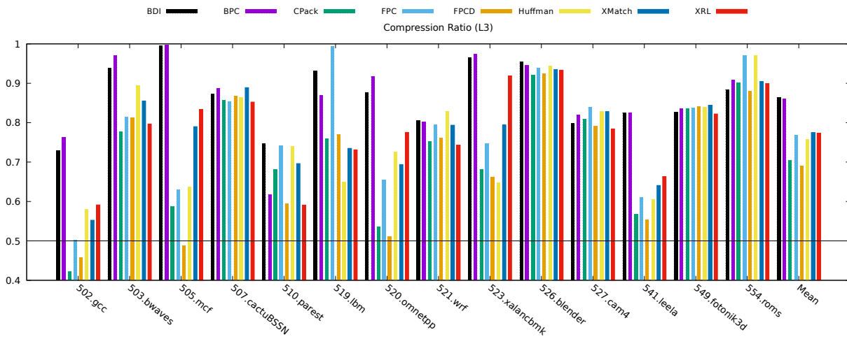
Figure 5.1 – Average compression ratio of SPEC 2017 workloads for multiple state-of-the-art cache compression methods applied to the LLC.
