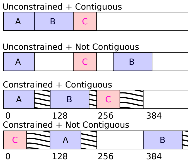
Figure 2.4 – Placement of compressed block C in a cache entry containing compressed blocks A and B, under different configurations. Stripes are wasted space.
