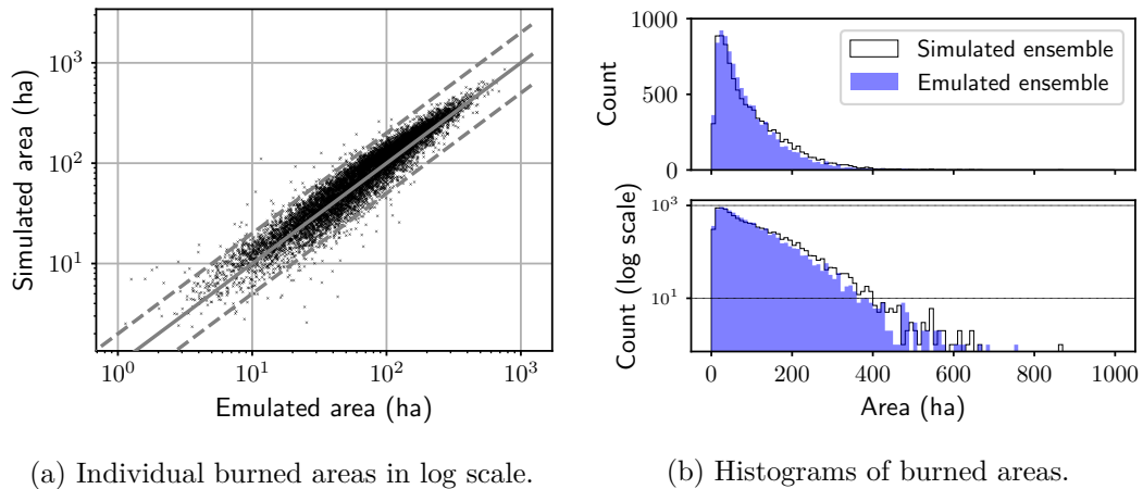
Figure IV.10. – Comparison between the ensemble of burned areas simulated by ForeFire for the fire case of Calenzana and their emulated counterparts. (a) The solid gray line corresponds to a perfect match and the dotted lines correspond to an error by a factor of 0.5 and 2. (b) Black contour: histogram of simulated areas; blue surface: histogram of emulated areas. Both top and bottom figures represent the same distributions, they share the same abscissa axis but the bottom figure has its ordinate in log scale.
