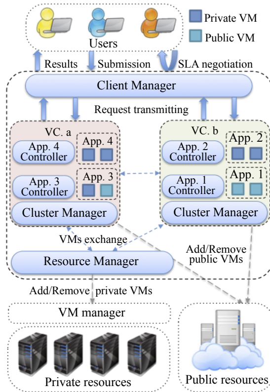
Figure 2.4: Meryn architecture
