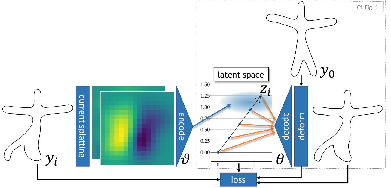
Figure 9.2: Global architecture of the diffeomorphic auto-encoder (DAE). An observation y_i is encoded as a normal probability distribution, from which is sampled a latent representation z_i \in \mathbb{R}^n . The latent-space segment [0, z_i] is then decoded into a dynamic velocity field, which is integrated into a diffeomorphism of the ambient space \mathbb{R}^d . This deformation is applied to a template shape y_0 to produce a reconstruction of the original shape y_i . The parameters of the encoder \vartheta , of the decoder \theta , and the template shape y_0 are estimated by stochastic gradient descent. To encode meshes, a preliminary current-splatting is performed before feeding y_i to the network.
