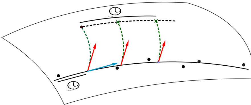
Figure 2.2: Time-reparametrized exp-parallelization of a reference geodesic model. The black dots are the observations, on which are fitted a geodesic regression (solid black curve, parametrized by the blue arrow) and a matching (leftmost red arrow). The red arrow is then parallel-transported along the geodesic, and exponentiated to define the exp-parallel curve (black dashes).
