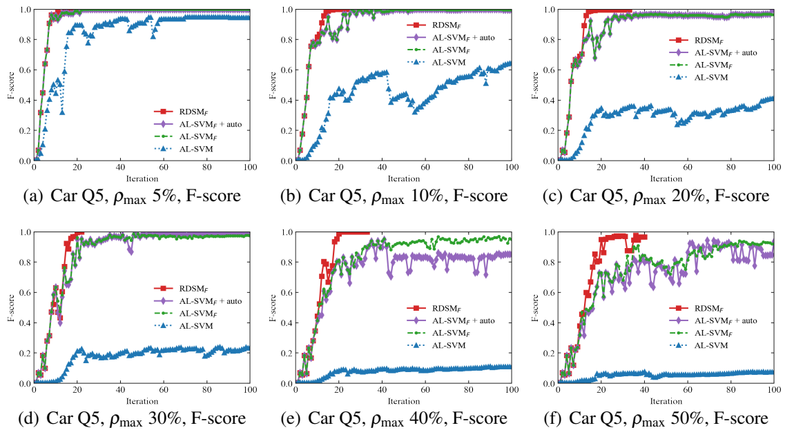
Figure 5.18: Comparison of \mathbf{RDSM}_F , \mathbf{AL-SVM}_F + \mathbf{auto} , \mathbf{AL-SVM}_F , and \mathbf{AL-SVM} for Car Q5
