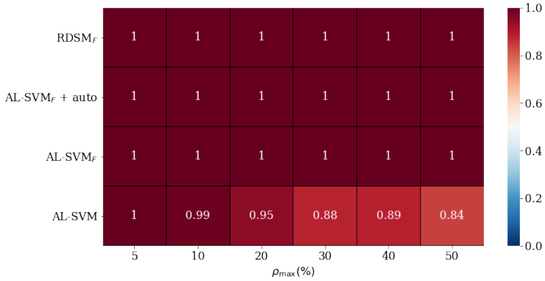
Figure 5.17: Maximum F-scores of \mathbf{RDSM}_F , \mathbf{AL-SVM}_F + \mathbf{auto} , \mathbf{AL-SVM}_F , and \mathbf{AL-SVM} over all Car queries at iteration 100
