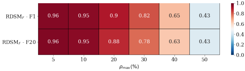
Figure 5.13: Averaged F-scores of \mathbf{RDSM}_F -F1 and \mathbf{RDSM}_F -F20 over all SDSS queries at iteration 200
