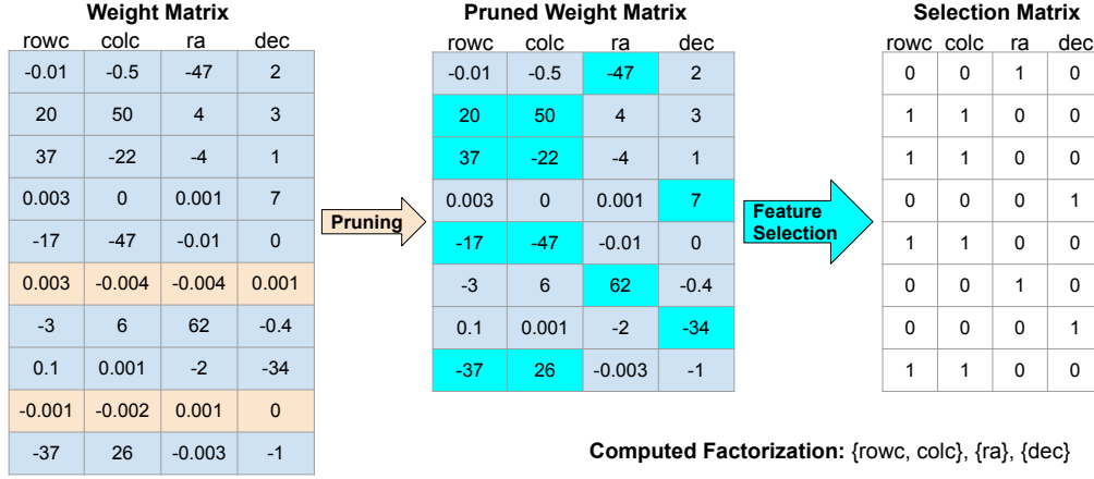
Figure 6.3: Example of our subspace and feature selection procedure over a 10-subspaces penalized FLM trained on SDSS 05. We also display the computed factorization (without duplicates), which is identical to the user’s own decomposition. Each row represents a different subspace, and each column a feature. Subspace pruning uses \epsilon_{zero} = \epsilon_{prob} = 0.01 .
