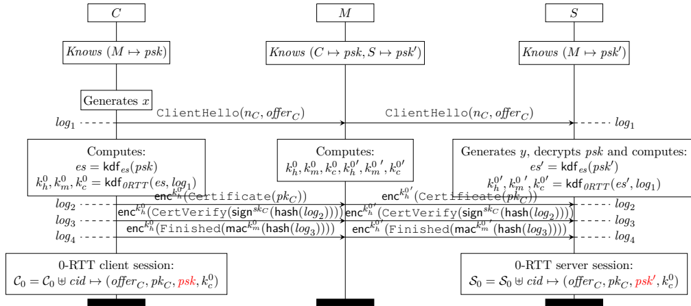
Figure B.3: Credential Forwarding Attack on PSK-based 0-RTT Client Authentication in Draft-12. This attack motivates the use of PSK binders—using psk to MAC the ClientHello )—in Draft-18.
