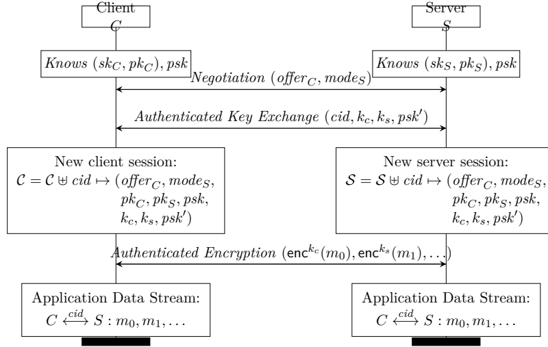
Figure 2.1: TLS Protocol Structure.
