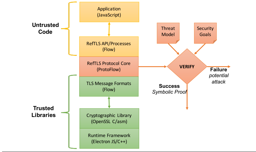
Figure 5.6: RefTLS Architecture.
