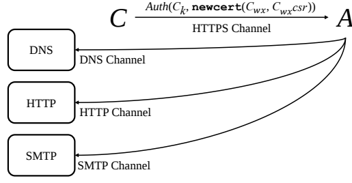
Figure 4.3: Channels overview.
