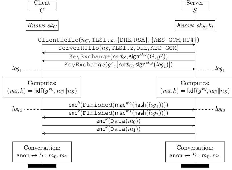
Figure 2.4: TLS 1.2 (EC)DHE handshake, no client authentication.
