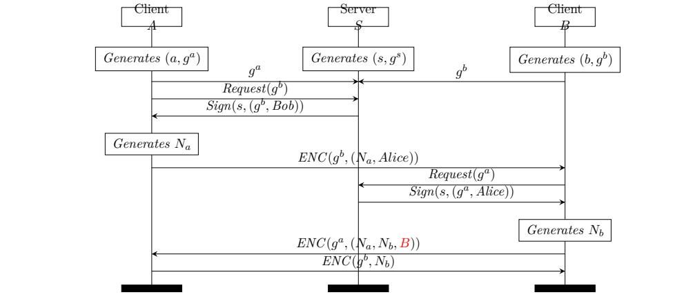
Figure 2: The Needham Schroeder Public-Key Protocol. This simple protocol, first described in 1978, was not broken until 1995 when a man-in-the-middle attack was discovered using automated formal verification in the symbolic model. By adding the component highlighted in red, the vulnerability can be addressed.
