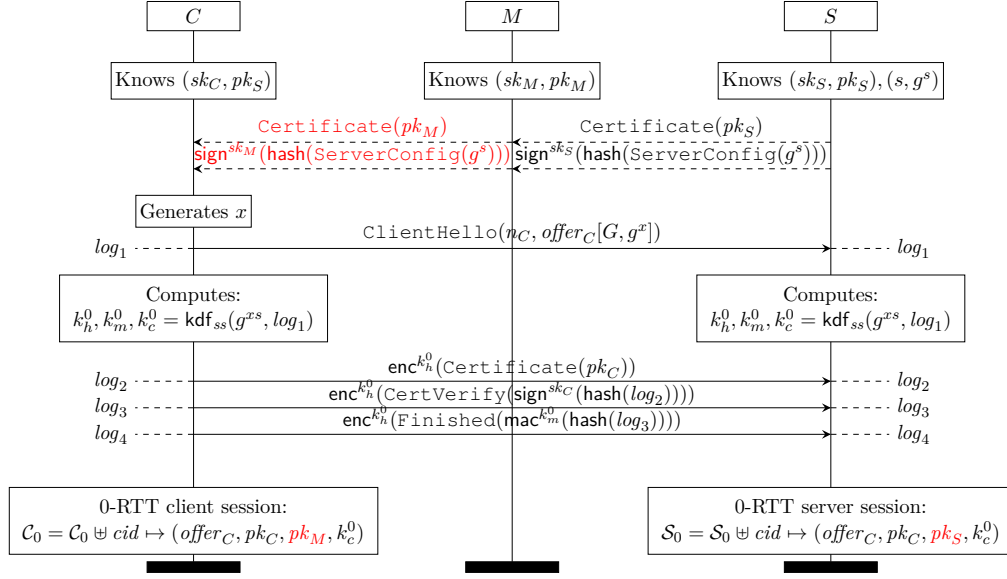
Figure B.2: Unknown Key Share (UKS) Attack in QUIC, OPTLS and on TLS 1.3 Draft-12 if the server’s certificate is not added to \log_1 . The figure shows how a man-in-the-middle can exploit the UKS to mount a credential forwarding attack on 0-RTT client authentication. This attack led to the inclusion of Certificate and ServerConfig in the 0-RTT handshake hash in Draft-7.
