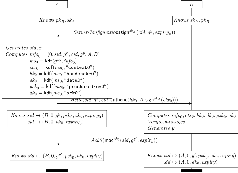
Figure B.5: The New Messaging Protocol: Start session with DH 0-RTT
