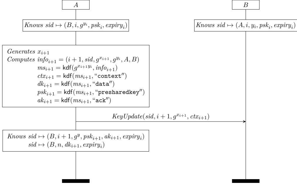
Figure B.7: The New Messaging Protocol: Key Refresh
