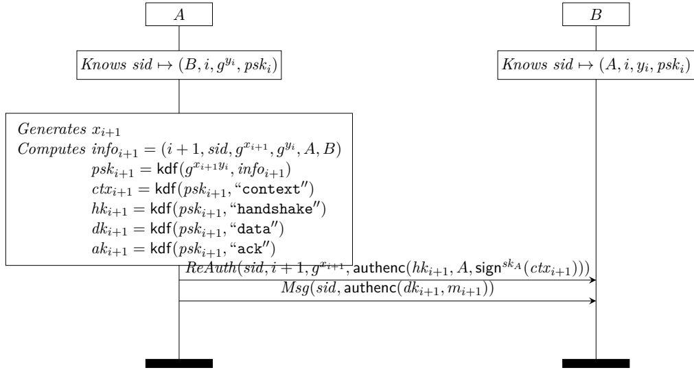
Figure B.8: The New Messaging Protocol: Re-authentication
