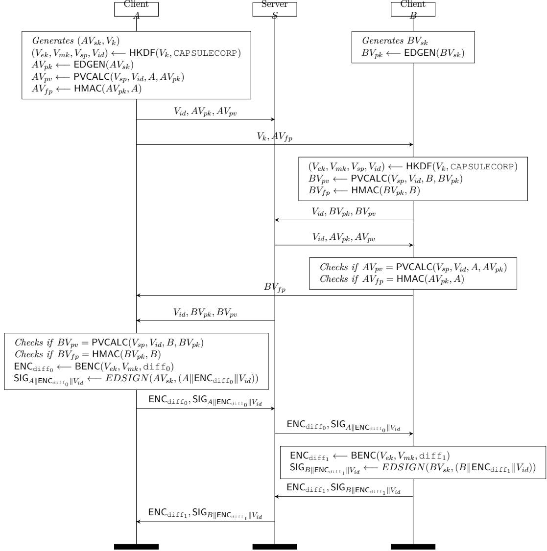
Figure 6.1: Capsule protocol session network messages. Here, A initiates a session with S and then communicates session key V_k and her own fingerprint AV_{fp} to B out of band. After B joins and all checks pass, A commits an example encrypted diff, \mathbf{diff}_0 and B follows up with an example diff \mathbf{diff}_1 . More involved sessions can include clients C , D , etc. with a non-deterministic diff commit schedule.
