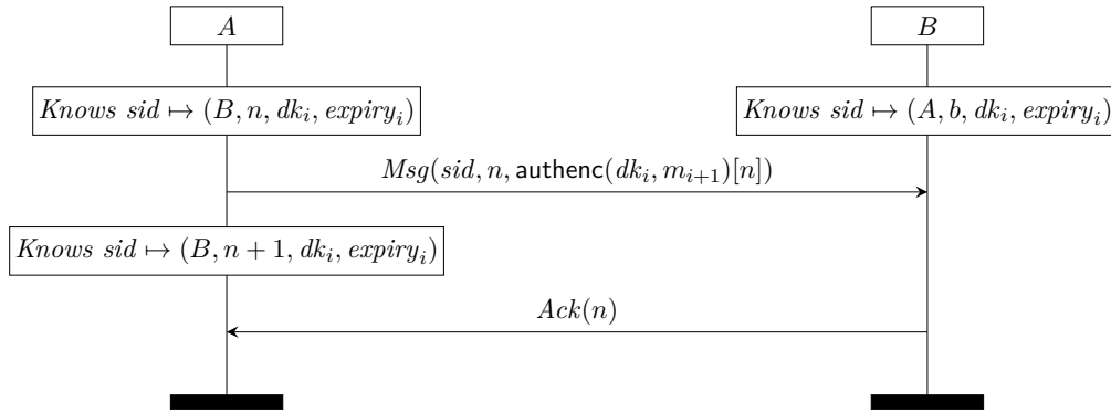
Figure B.6: The New Messaging Protocol: Sending Data
