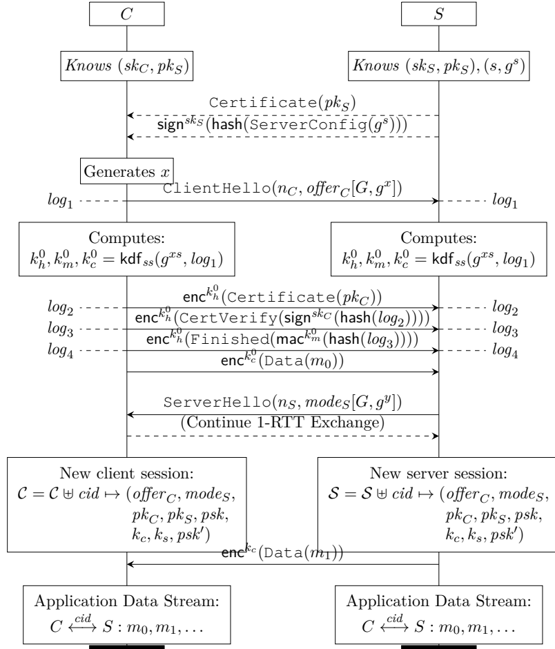
Figure 2.6: DH-based 0-RTT in TLS 1.3 Draft-12, inspired by QUIC and OPTLS.
