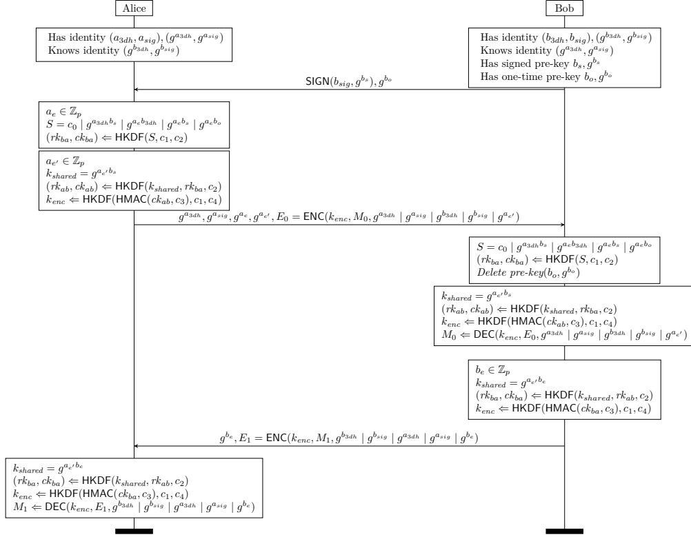
Figure 1.2: SP, a variant of Signal with minor differences. Alice requests a signed pre-key from Bob (via the server) and sends an initial message M_0 . Bob accomplishes his side of the key exchange and obtains M_0 . Bob later sends his reply M_1 , illustrating the Axolotl ratchet post-AKE. We ignore the hash-based ratchet that occurs when two consecutive messages are sent in the same direction. c_i refers to various constants found throughout the protocol.
