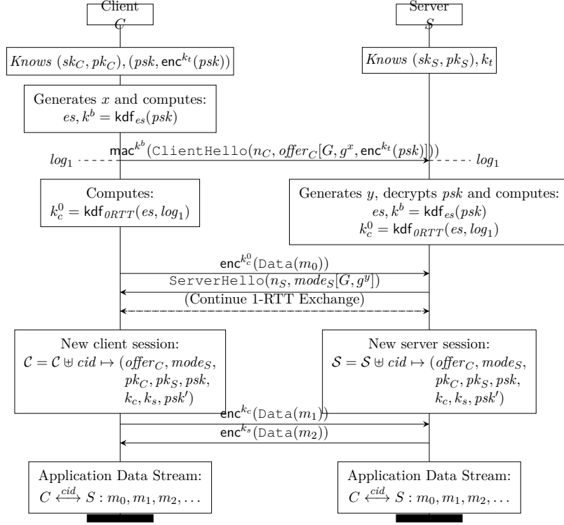
Figure 2.7: TLS 1.3 Draft-18 PSK-based Resumption and 0-RTT.
