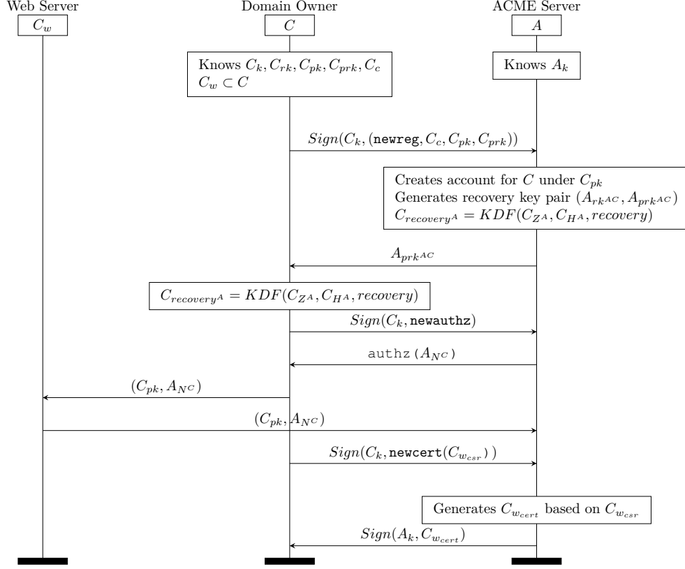
Figure 4.4: ACME draft-1 protocol functionality for C account registration, recovery key generation, and validation with certificate issuance for C_w . This chart demonstrates validation via an HTTP identifier. In draft-3 and above, the HTTP challenge (C_{pk}, A_{NC}) is replaced with \text{Sign}(C_k, (C_{pk}, A_{NC})) .
