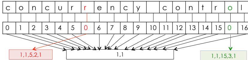
Figure 4.5: LOGOOTSPPLITSTRING representation
