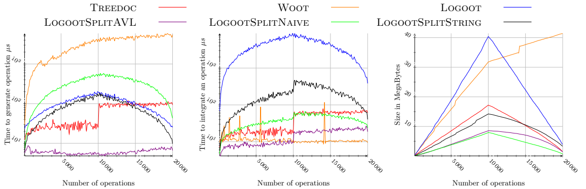
(a) Generation time (b) Remote integration time (c) Memory occupation
