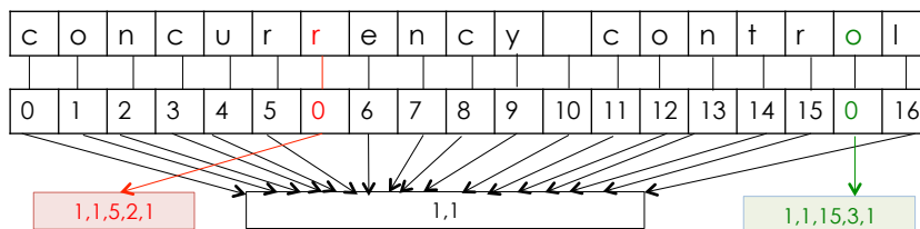
Figure 4.5: LOGOOTSPPLITSTRING representation
