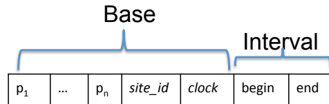
Figure 4.2: LogootSplit identifier
