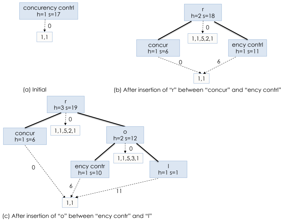
Figure 4.6: LOGOOTSPLITAVL representation
