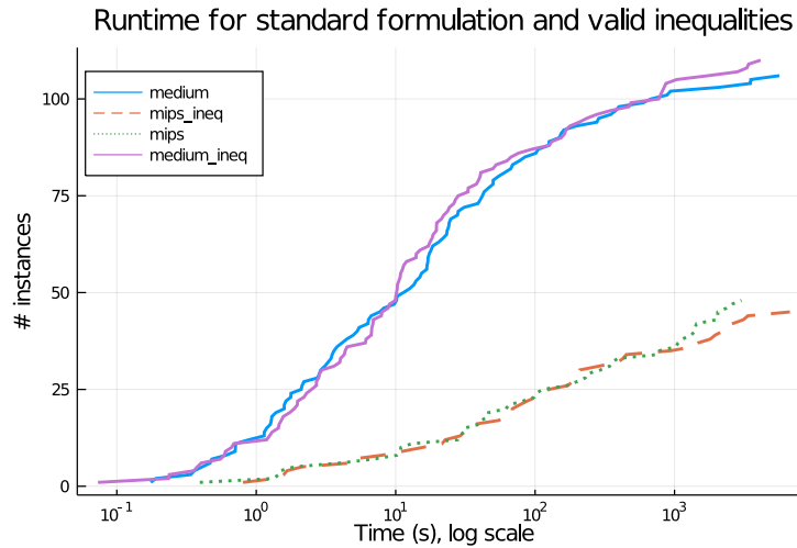
Figure 6.9 Runtime for MIPS and medium instances with and without valid inequalities.
