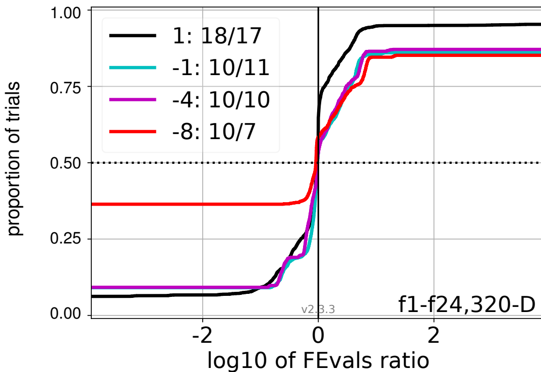
Figure 4.5: ECDF of runtime ratios of LMCMA divided by VxD-CMA for all functions in dimension 320 to reach target values 10^k with k given in the legend; all trial pairs for each function. Pairs where both trials failed are disregarded, pairs where one trial failed are visible in the limits being > 0 or < 1 . The legend also indicates, after the colon, the number of functions that were solved in at least one trial (LMCMA first).
