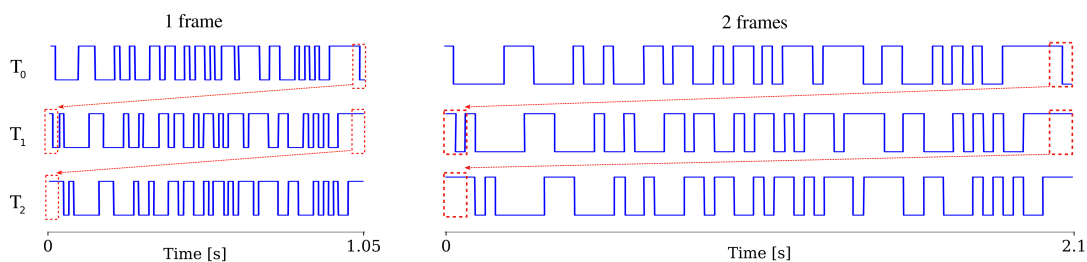
FIGURE 3.8 – Illustration of the circular-shift process for the stimulus sequence for the first 3 targets. On the left, the stimulus sequences have a frame rate of 60 Hz (1 bit = 1 frame) and on the right, a frame rate of 30 Hz (1 bit = 2 frames). The figure shows the stimulation sequence for the target T_0 , for the target T_1 , circularly shifted with a time lag \tau_s with respect to T_0 and for the target T_2 , circularly shifted with a time lag \tau_s with respect to T_1 . The red dash boxes indicate the time lag \tau_s corresponding to the number of frames, listed in Table 3.3.
