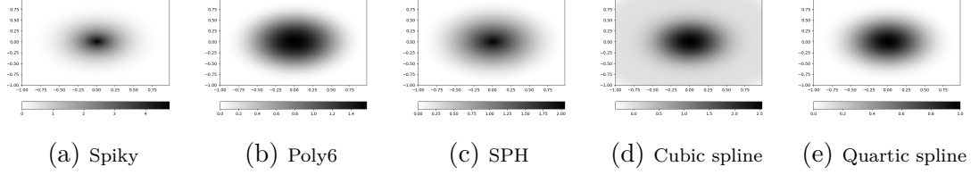
Figure 3.4: 2D kernels
