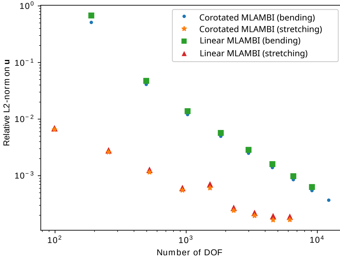
Figure 3.13: Relative L2-norm of the displacement error between the solution with n Degrees Of Freedom (DOF) and the solution with (n-1) DOF for stretching and bending scenarios, using a linear elasticity material with and without our corotated approach.
