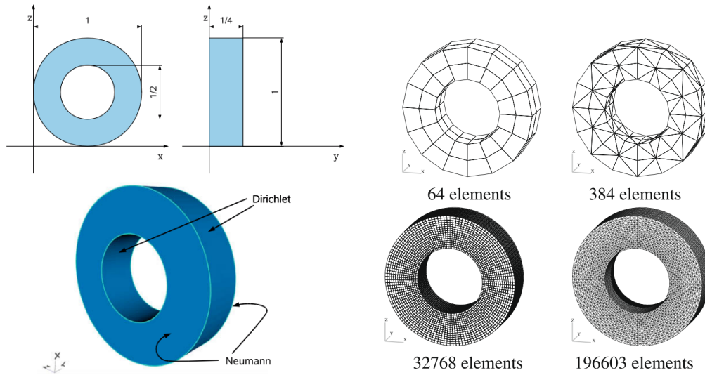
(a) Geometry and boundary conditions of the problem. (b) Coarser and finer hexahedral (left) and tetrahedral (right) meshes.
