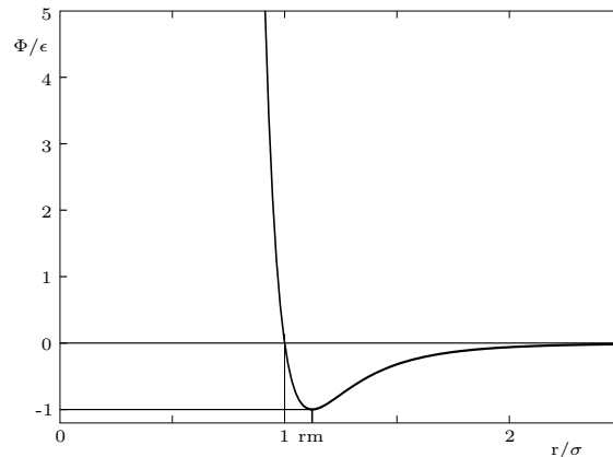
Figure 3.1: Lennard-Jones potential \phi_{LJ}(r) = \frac{B}{r^{12}} - \frac{A}{r^6} with n = 12 , m = 6 , \epsilon = \frac{B^2}{4A} and \sigma = \sqrt[6]{\frac{A}{B}} . Here, the scalar parameters A and B defines the attraction-repulsion behavior, and r denotes the distance between two particles.
