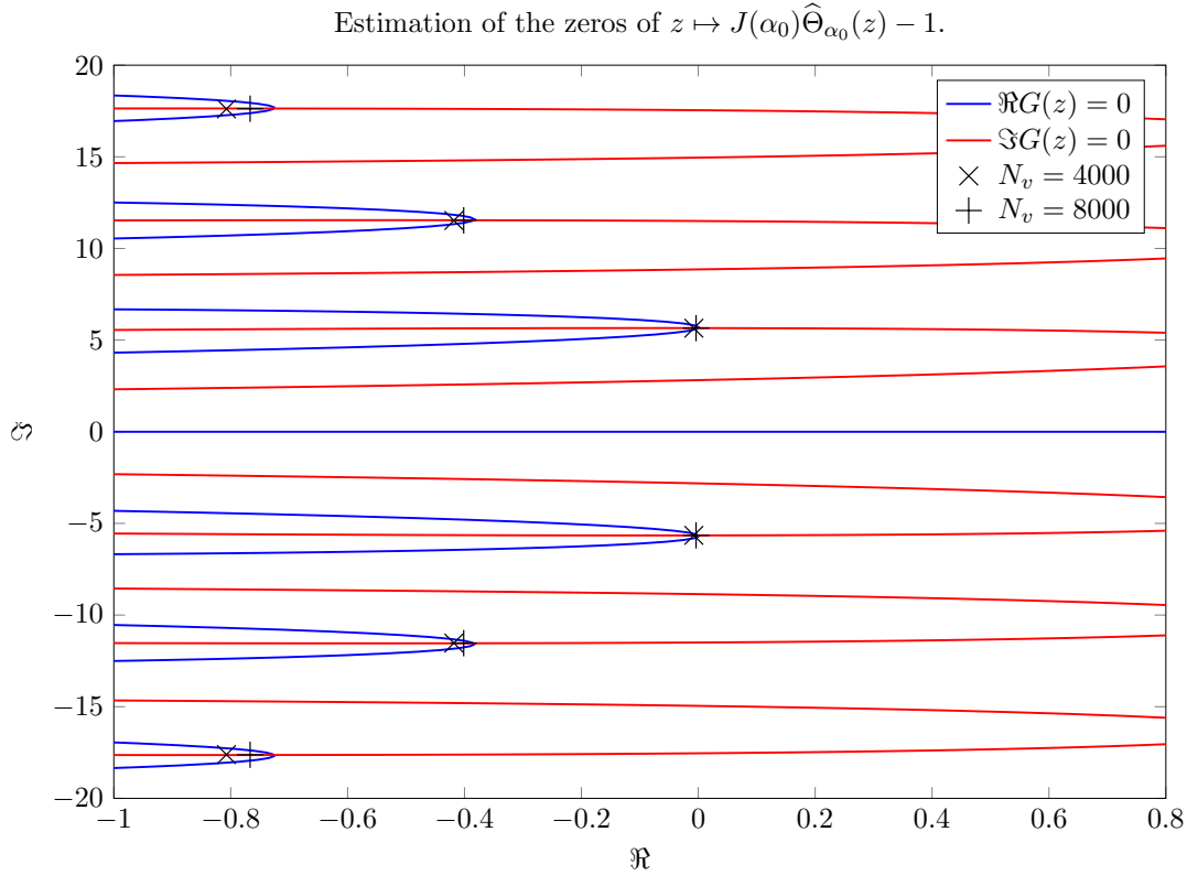
Figure 6.7: Estimations of the zeros of z \mapsto J(\alpha_0)\hat{\Theta}_{\alpha_0}(z) - 1 using the algorithm described in Section 6.4.2. The exact setting is described Section 6.4.2. We used v_{\max} = 2 and N_v \in \{4000, 8000\} . Let G(z) be the function defined by (6.7). The zeros of G match with the zeros of z \mapsto J(\alpha_0)\hat{\Theta}_{\alpha_0}(z) - 1 . The blue curve corresponds to the solution of the equation \Re G(z) = 0 , while the red curve corresponds to \Im G(z) = 0 . Hence, the points where the two curves intersect are the “true” zeros of G . With our choice of parameters, it holds that \pm i2\pi(1 - 0.1) \approx \pm i5.655 are a pair of zeros of G . With N_v = 8000 , the algorithm computes the pair of zeros -0.004 \pm i5.653 . Overall the error is of order 4 \cdot 10^{-3} .
