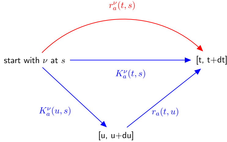
Figure 2.1: The probability that Y_{\cdot,s}^{a,\nu} spikes between t and t + dt is, by definition, approximately equals to r_a^\nu(t, s)dt . Either such spike is the first (and so there are no spikes between s and t ), which occurs with probability K_a^\nu(t, s)dt . Either there is a first spike, say between u and u + du for some u \in (s, t) . This happens with probability K_a^\nu(u, s)du and the process is reset to 0 at this time u , such that the required probability is K_a^\nu(u, s)r_a(t, u)dudt . Integrating over all u \in (s, t) , we find the Volterra integral equation (2.12). We refer to the proof of Proposition 2.24 for more details.
