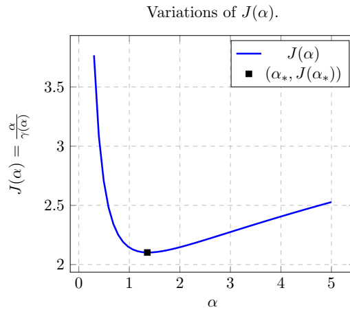
Figure 6.1: Plot of the function \alpha \mapsto J(\alpha) = \frac{\alpha}{\gamma(\alpha)} , for b(x) = -x and f(x) = x^2 . We proved in Proposition 6.1 that this function is decreasing on (0, \alpha_*] and increasing on [\alpha_*, \infty) .
