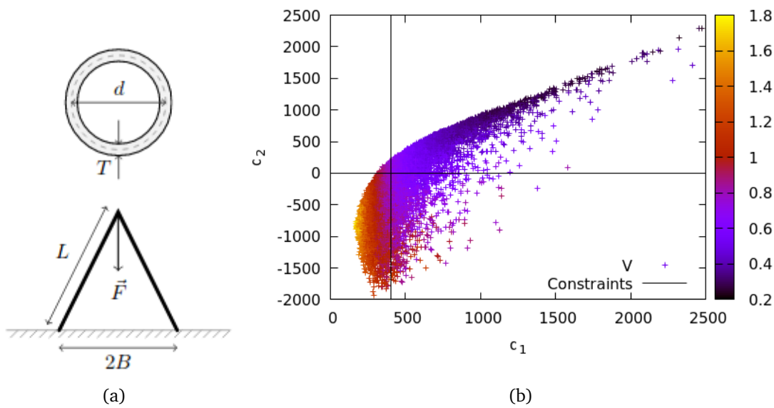
Figure V.1 (a) Schematic representation of the two bars, with bar section above (from [Baudouin, 2012]). (b) Representation in the objective/constraints space, constraints in abscissa and ordinate, objective in color.
