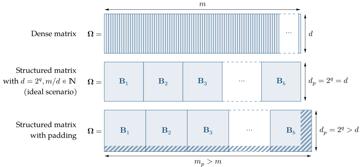
Figure 5.3: Construction of the whole matrix of frequencies, with the dense approach (top), with structured blocks when d is a power of 2 (middle), and with structured blocks and padding (bottom). The hatched area represents the “unused” part of the construction when using padding.
