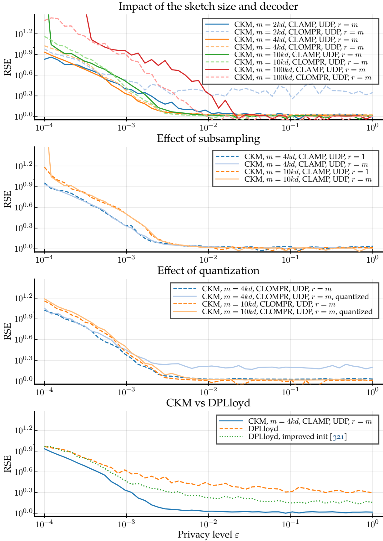
Figure 9.4: Privacy-utility tradeoff on synthetic data for \varepsilon -UDP. Parameters: k = d = 10 , n = 10^7 . Data generated according to (4.5) with separation factor s = 2.5 . Medians over 50 trials (except for m = 100kd where fewer trials are used).
