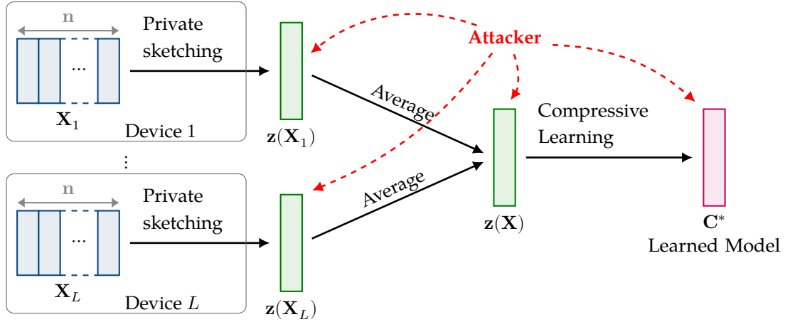
Figure 7.1: Attack model. The dataset is distributed between L devices, each computing and releasing publicly a sub-sampled sketch \mathbf{z}(\mathbf{X}_i) .
