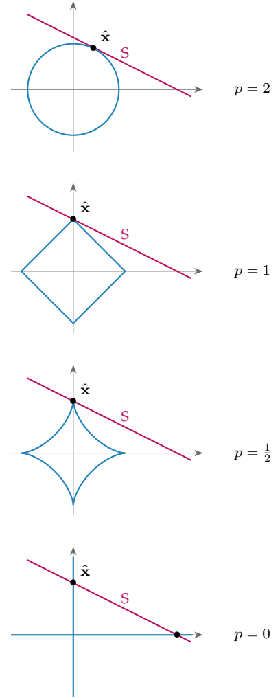
Figure 2.2: Standard l_p (pseudo-)norms in dimension 2. Here S represents the linear constraint induced by the observations. The blue curves show for each p > 0 the first iso-line of the l_p (pseudo-)norm which intersects with S , giving the solution \hat{\mathbf{x}} of smallest l_p norm which satisfies the linear constraint. For p = 0 , the blue set is \Sigma_1 . All l_p pseudo-norms for p \leq 1 somehow induce sparsity, but only l_1 yields a convex optimization problem. 7 LASSO stands for “least absolute shrinkage and selection operator”.
