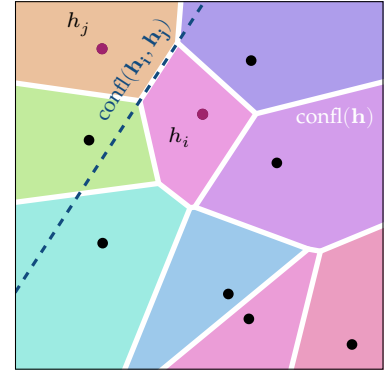
Figure 10.2: Illustration of Definition 10.8 when h is a union of k points. We obtain a Voronoi diagram, whose colored cells correspond to the territories associated to the points (h_i)_{1 \leq i \leq k} . The blue dashed line corresponds to the conflict set between h_i and h_j (points in purple), and \text{confl}(h) is represented in white.
