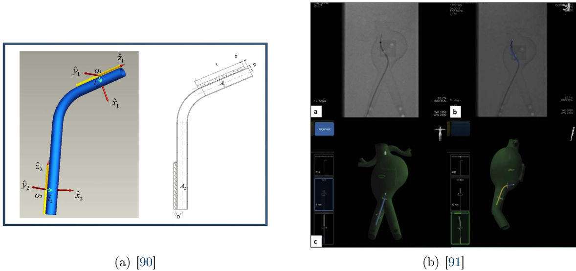
Figure 2.15: (a) [90] Representation of a traditional catheter with two sensor coils (yellow cylinder). (b) [91] Comparison between classic fluoroscopic images against 3D virtual reality images generated with 3D EM sensors for catheter position and model of the anatomy.
