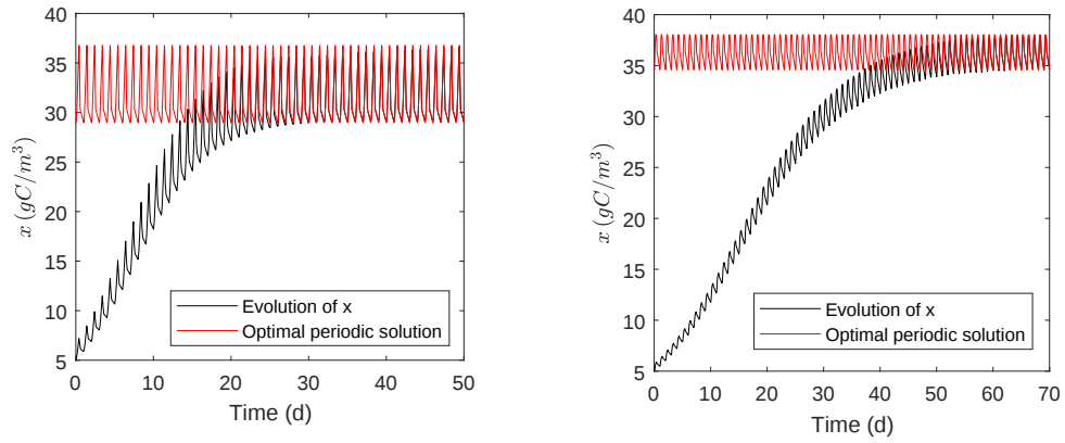
Figure 7.3: Comparison of the optimal 1-day periodic microalgae concentration and the evolution of the microalgae with a low initial concentration when the periodic 1-day optimal periodic control is applied. Left. Culture without background turbidity. Right. Culture with background turbidity.
