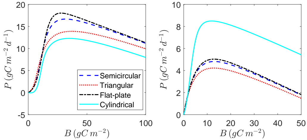
Figure 3.9: Productivity as a function of the biomass concentration per illuminated surface. A. I_{in} = 1000 \mu mol m^{-2} s^{-1} B. I_{in} = 50 \mu mol m^{-2} s^{-1} . We consider p given by (3.25) with the kinetic parameters of C. vulgaris given in Table 2.1. The other parameters are taken to be k = 0.2 m^2 gC^{-1} , m = 0.1 d^{-1} , and K_{bg} = 0 .
