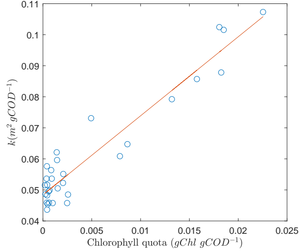
Figure 8.1: Correlation between the chlorophyll quota \theta and the specific light attenuation coefficient of microalgae k . Experimental data is taken from the work of [15]. The linear regression is given by k = 2.5459 \times \theta + 0.0484 .
