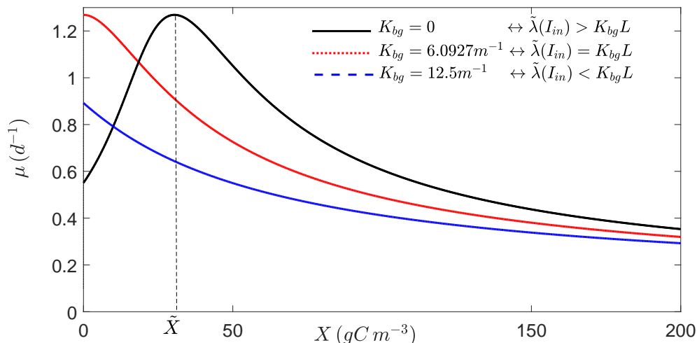
Figure 3.7: Plot of the AGR as a function of X . We consider p given by (3.25) with the kinetic parameters of C. vulgaris given in Table 2.1. The other parameters are taken to be I_{in} = 500 \mu \text{ mol m}^{-2} \text{ s} , k = 0.2 \text{ m}^2 \text{ gC}^{-1} , L = 0.4 \text{ m} .
