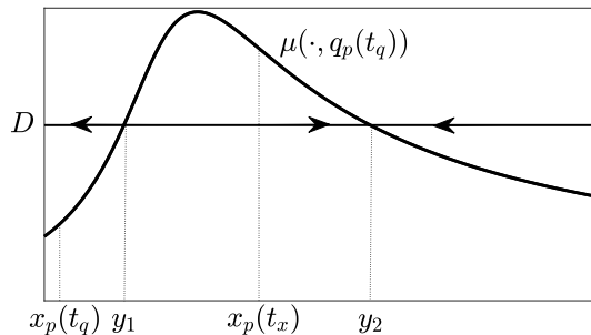
Figure 5.2: Function y \mapsto \mu(y, q_p(t_q)) and illustration of the dynamics of (5.6)
