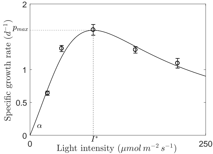
Figure 2.2: Carbon uptake rate (see (2.5)) for Chlorella vulgaris with experimental data from [51].
