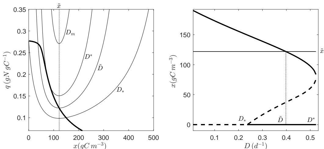
Figure 5.3: A. Intercepts of \Gamma_1 and \Gamma_2(D) for different dilution rates in the case 2. The bold line corresponds to \Gamma_1 . B. Bifurcation diagram of x with respect to D .
