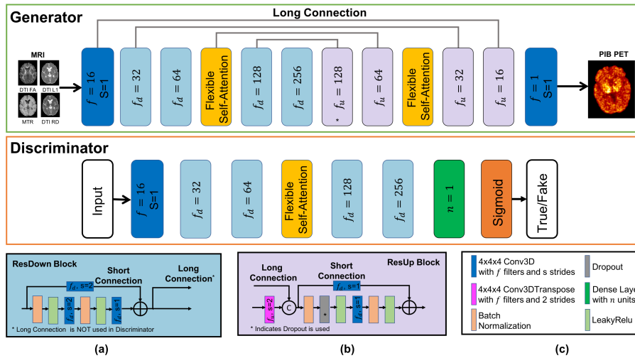
Fig. 4.2: The overall framework of the proposed CF-SAGAN. (a-c) Illustration of the different units and layers used in the Generator and the Discriminator. The values f_d, f_u, f indicate the number of feature maps in each unit and s is the stride number. The parameter n refers to the units number in the Dense layer. (For interpretation of the references to color in this figure legend, the reader is referred to the web version of this article.)
