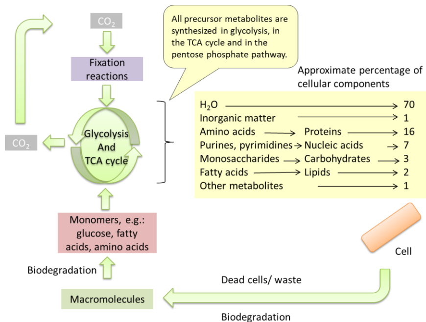
Figure 1-6: Global view of synthesis and degradation reactions of the cell
