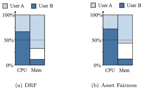
Figure 1.12: An example of 'DRF' and 'Asset fairness' allocations [4].
