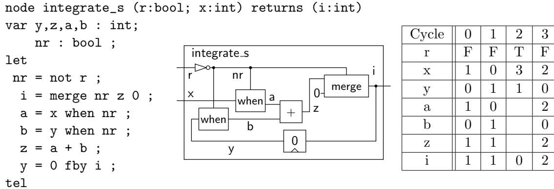
Figure 2.8: Conditional execution in Heptagon
