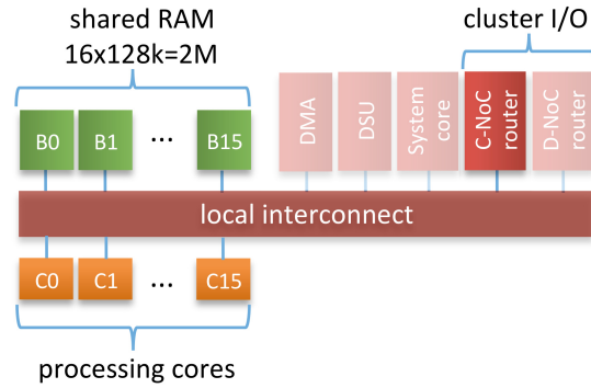
Figure 3.2: Structure of a Kalray MPPA 256 Bostan compute cluster
