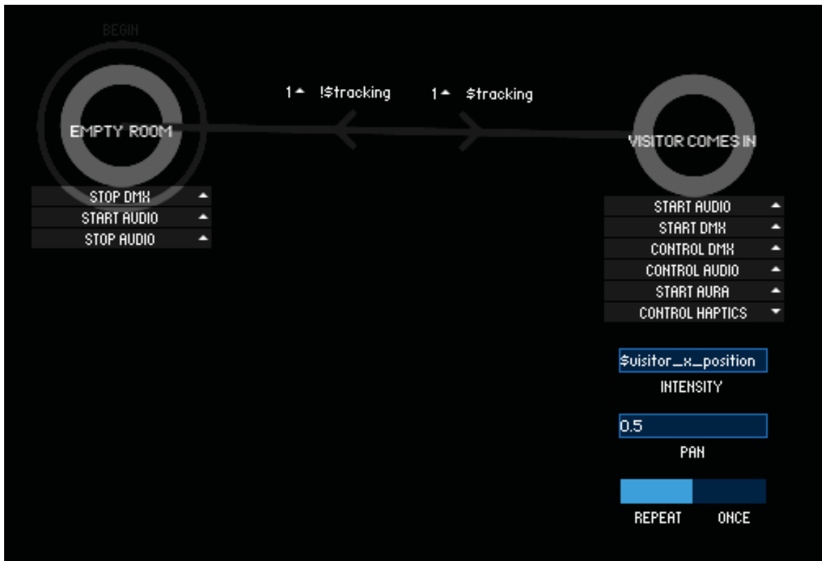
Fig. 5.1 ZenStates allows users to quickly prototype interactive environments by directly manipulating States connected together via logical Transitions . Tasks add concrete actions to states and can be fine-tuned via high-level parameters (e.g. ‘intensity’ and ‘pan’). Blackboard global variables (prefixed with the ‘$’ sign) can enrich tasks and transitions. © 2018 IEEE.
