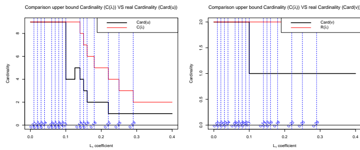
Figure 6: Behaviors of the cardinalities and their upper bounds, defined with corollary 2.1.1, for a simulation case, first component.
