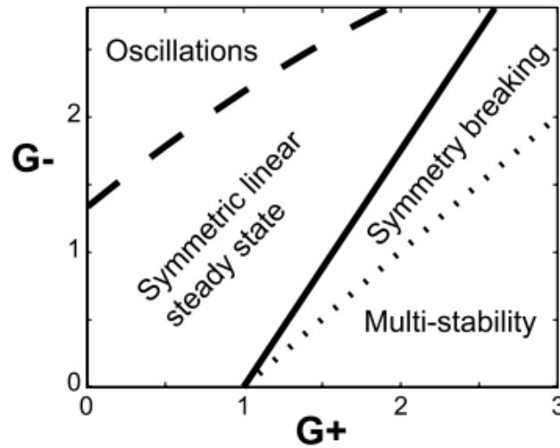
Figure 6.15: The phase diagram for the various dynamical regimes of the reduced model in (Leblois 2006) as a function of G_+ and G_- . Figure copied from (Leblois 2006)
